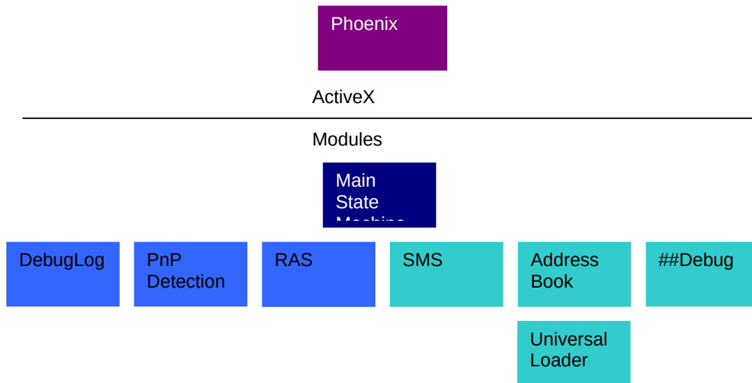
Figure 10: Module Design
