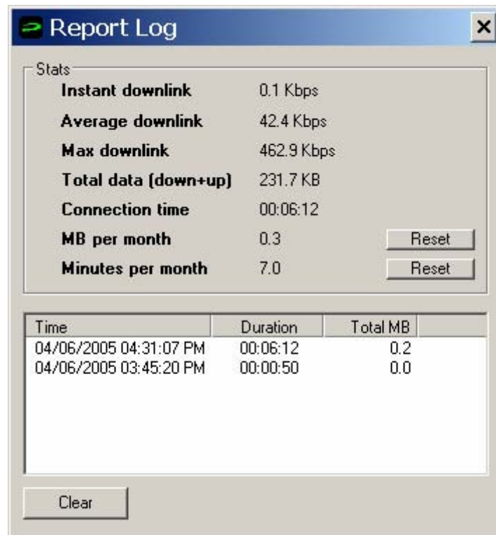
Figure 37: Report Log
