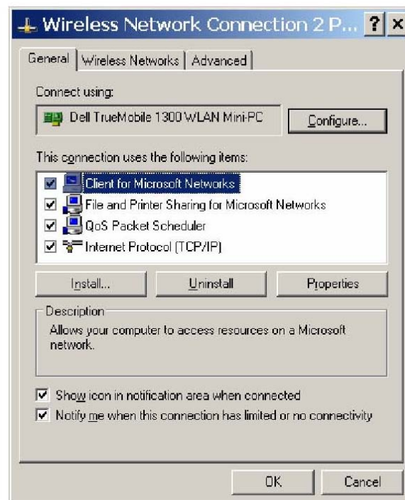
Figure 32: WAP Window
