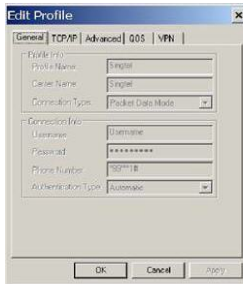
Figure 24: Profile Settings
