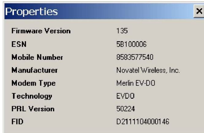
Figure 35: CDMA
