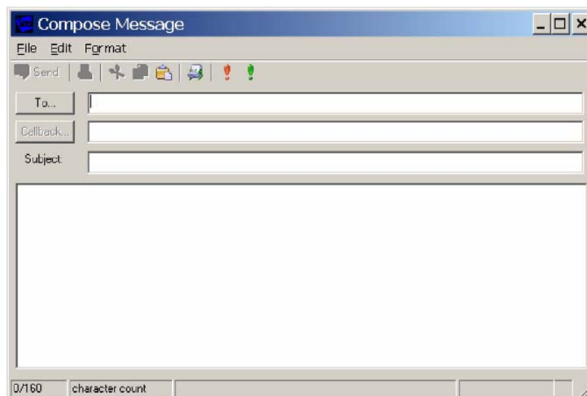
Figure 44: Compose Message
