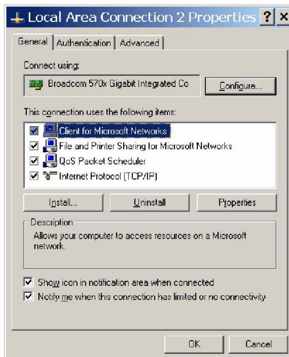
Figure 34: AP Window
