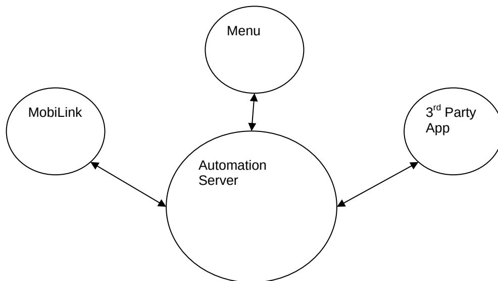
Figure 11: Automation Server
