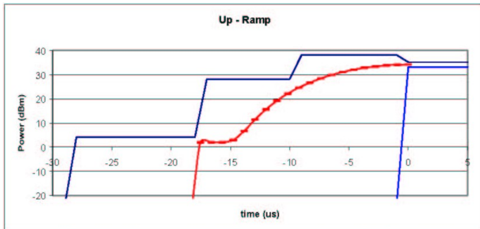
Figure 5: Up-ramp for Highest Power Levels
