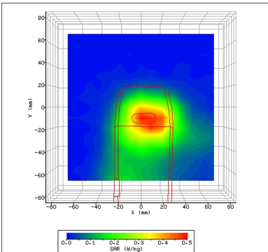
Figure 34: SAR Body Testing Results for the Novatel U730 Wireless PCMCIA Card in Rear Facing Phantom Position; Tested at 1880.0MHz (1900 GSM EDGE Middle Channel) with 10mm Separation – Host 1 used Report Number WS614714/01 Issue 1
