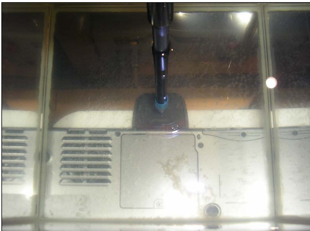
Figure 48: Positional Photograph of the Novatel U730 Wireless PCMCIA Card in Rear Facing Phantom Position using Host 3 – Dell Latitude D600; 14mm Separation Distance
