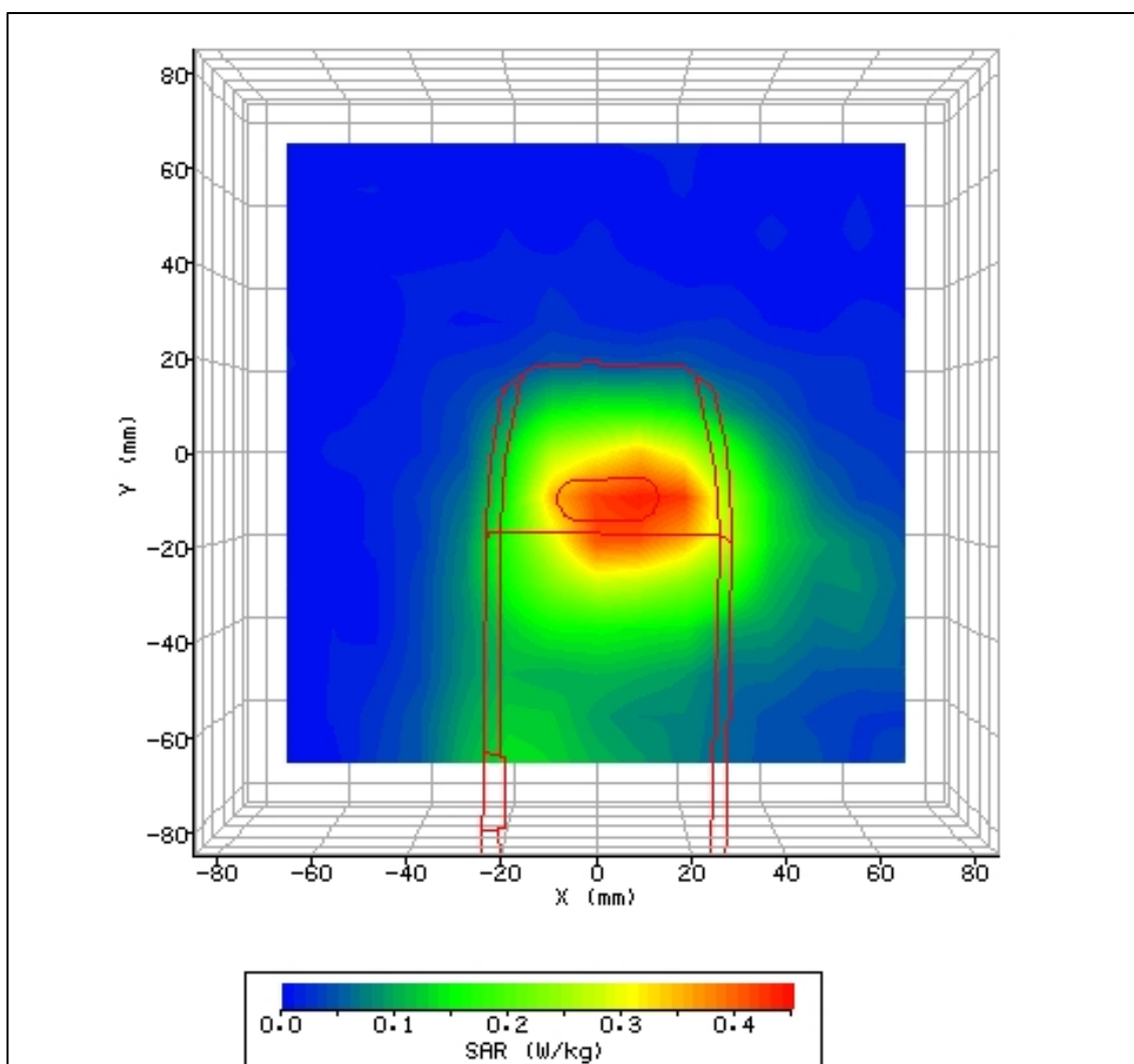
Figure 35: SAR Body Testing Results for the Novatel U730 Wireless PCMCIA Card in Rear Facing Phantom Position; Tested at 1850.2MHz (1900 GSM EDGE Bottom Channel) with 10mm Separation – Host 1 used Report Number WS614714/01 Issue 1 Page 48 of 71
