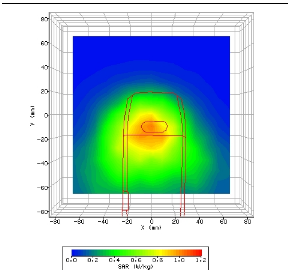
Figure 33: SAR Body Testing Results for the Novatel U730 Wireless PCMCIA Card in Rear Facing Phantom Position; Tested at 848.8MHz (850 GPRS Top Channel) with 14mm Separation – Host 3 used
