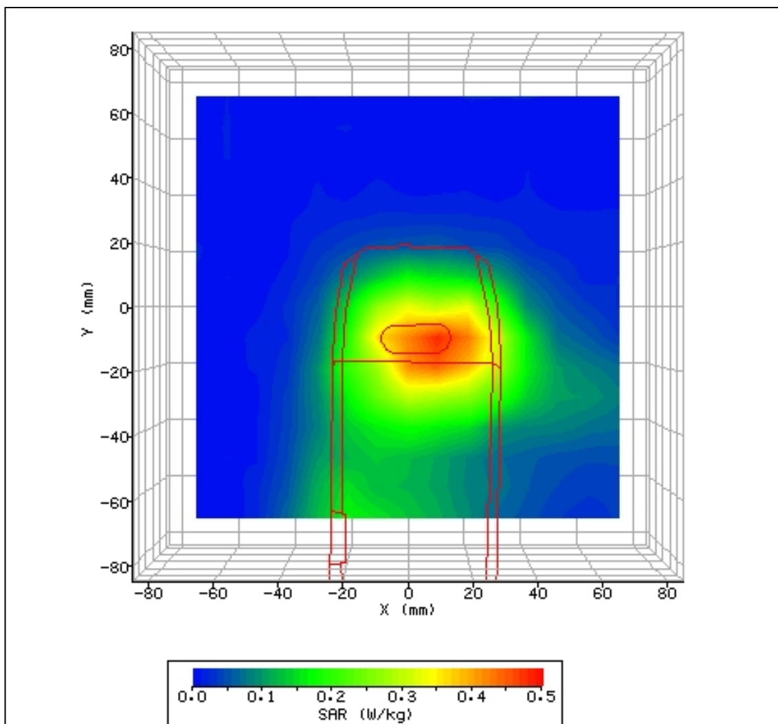
Figure 36: SAR Body Testing Results for the Novatel U730 Wireless PCMCIA Card in Rear Facing Phantom Position; Tested at 1909.8MHz (1900 GSM EDGE Top Channel) with 10mm Separation – Host 1 used Report Number WS614714/01 Issue 1 Page 49 of 71
