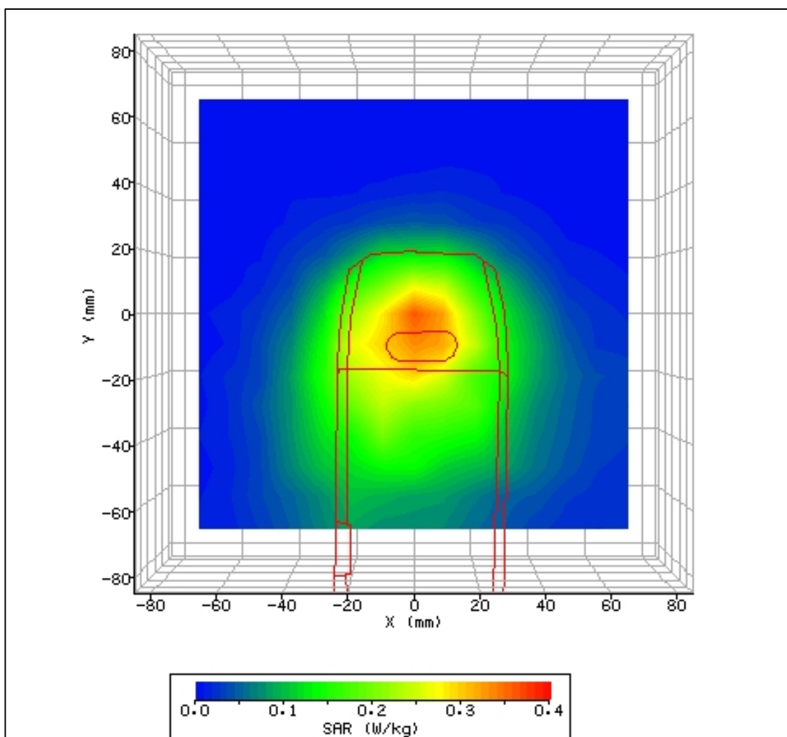
Figure 40: SAR Body Testing Results for the Novatel U730 Wireless PCMCIA Card in Rear Facing Phantom Position; Tested at 824.2MHz (850 GSM EDGE Bottom Channel) with 10mm Separation – Host 1 used Report Number WS614714/01 Issue 1 Page 53 of 71
