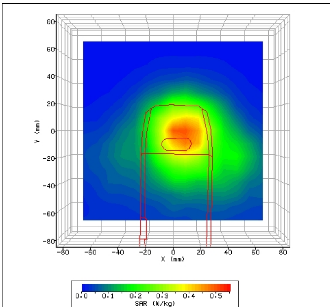
Figure 42: SAR Body Testing Results for the Novatel U730 Wireless PCMCIA Card in Rear Facing Phantom Position; Tested at 848.8MHz (850 GSM EDGE Top Channel) with 18mm Separation – Host 2 used
