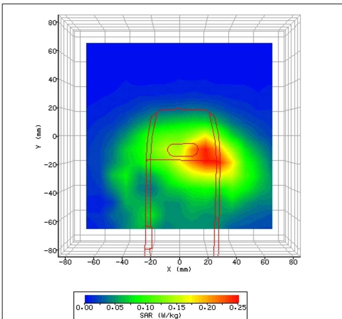
Figure 38: SAR Body Testing Results for the Novatel U730 Wireless PCMCIA Card in Rear Facing Phantom Position; Tested at 1909.8MHz (1900 GSM EDGE Top Channel) with 14mm Separation – Host 3 used Report Number WS614714/01 Issue 1
