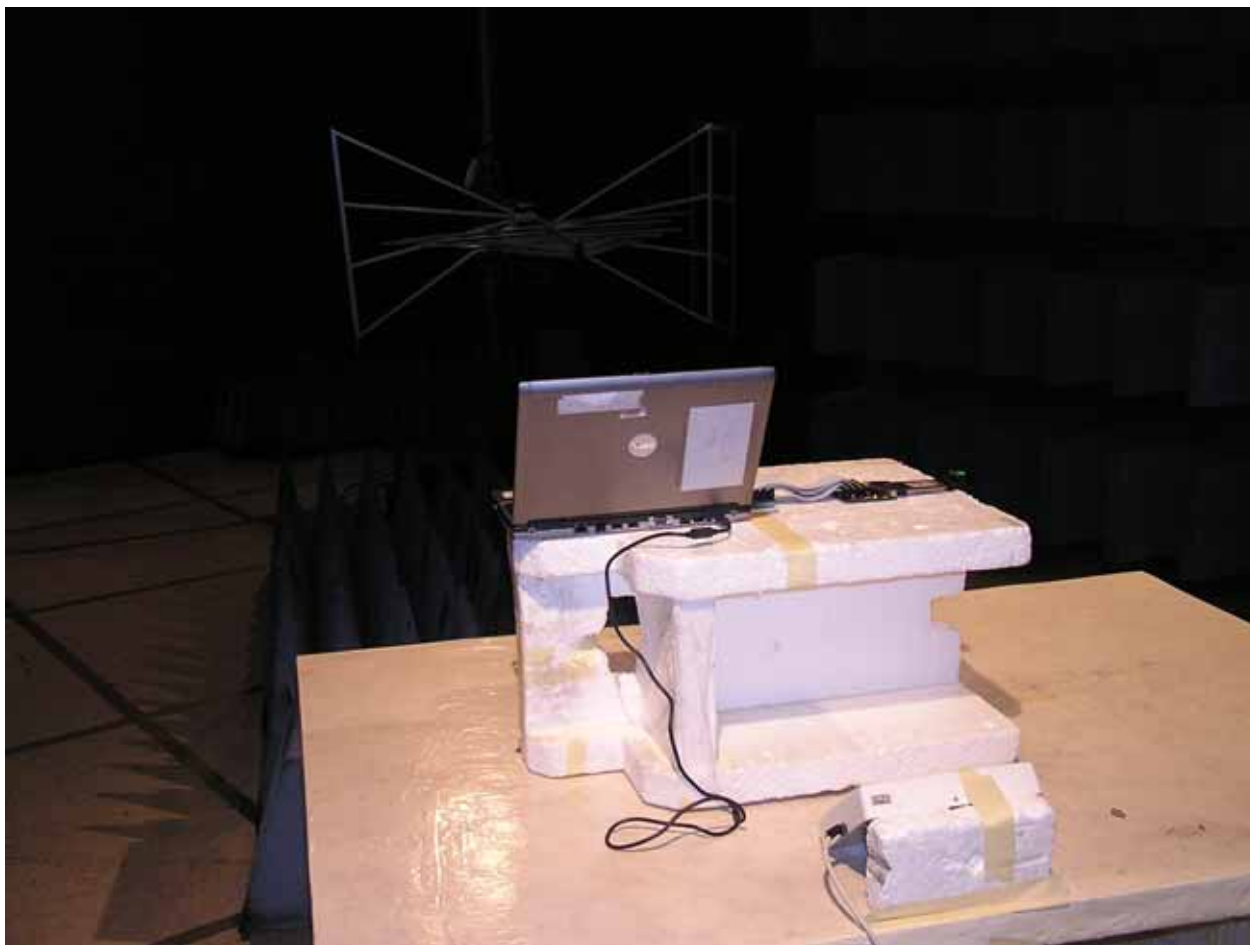
RADIATED EMISSIONS
