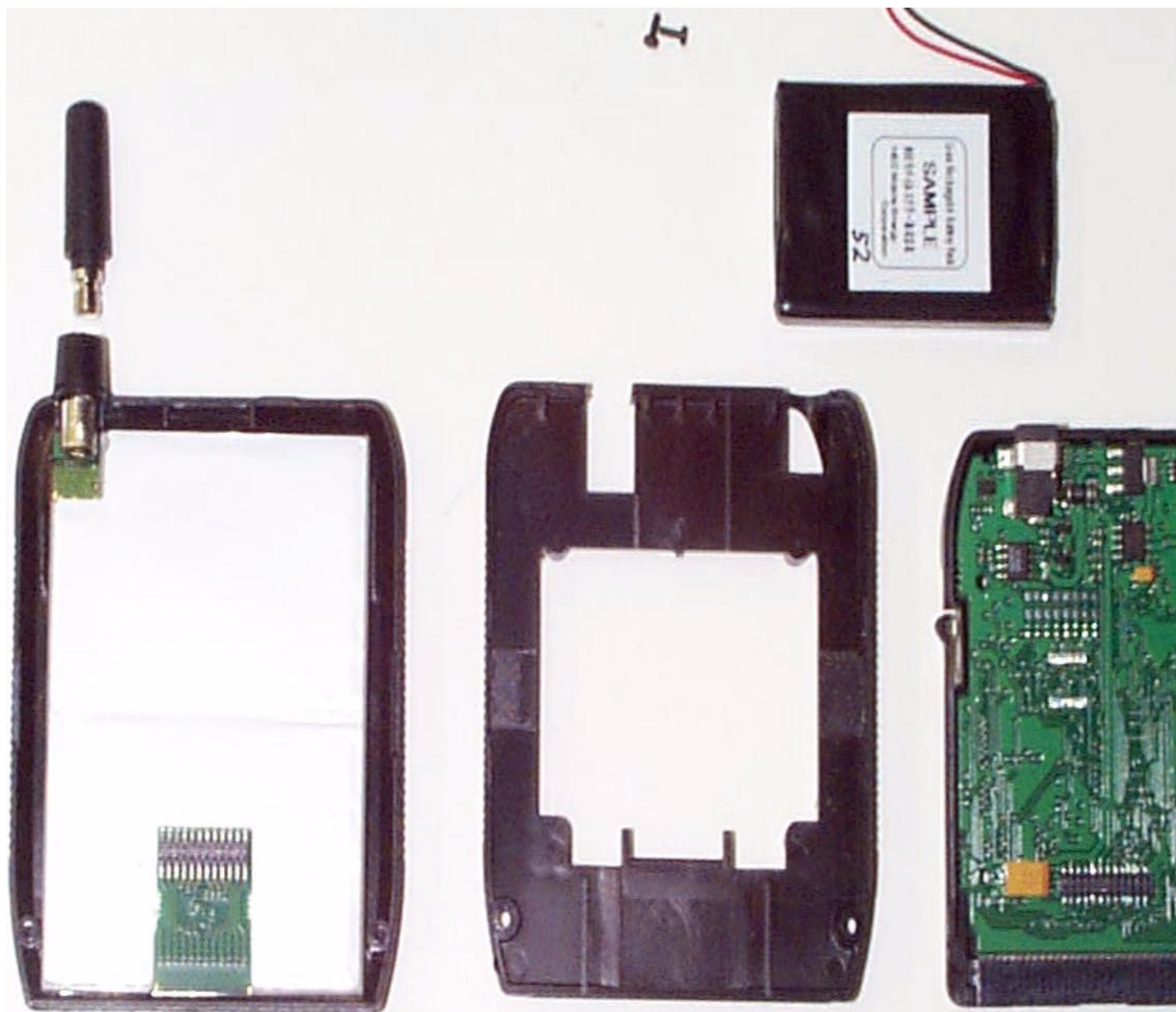
NBZNRM-6834 BATTERY REMOVED VIEW
