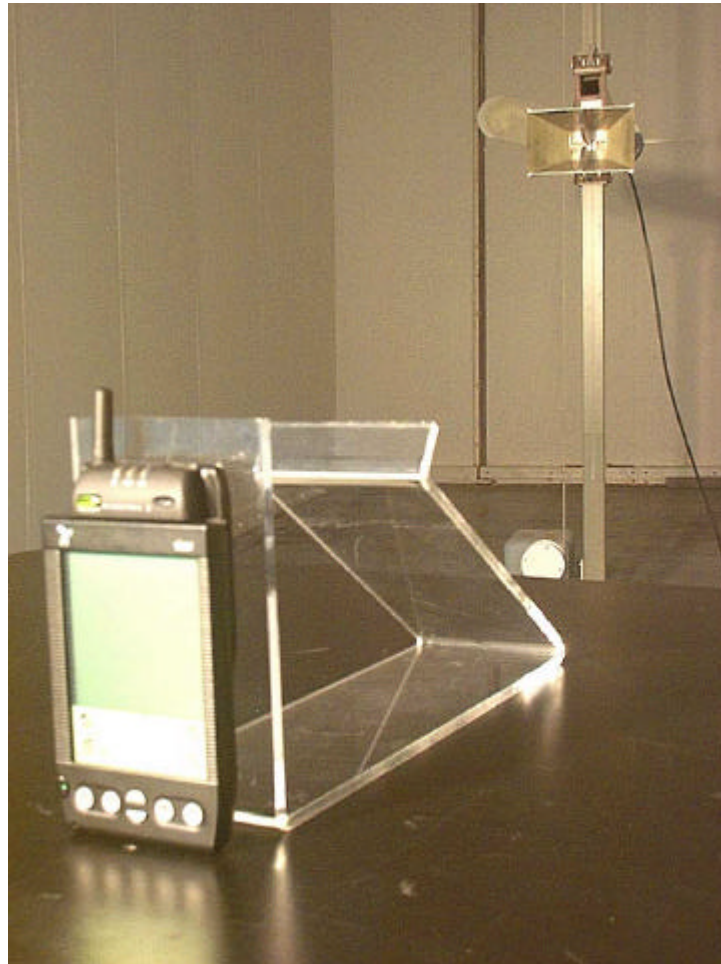
Spurious Measurements in OATS (for frequencies above 1 GHz)
