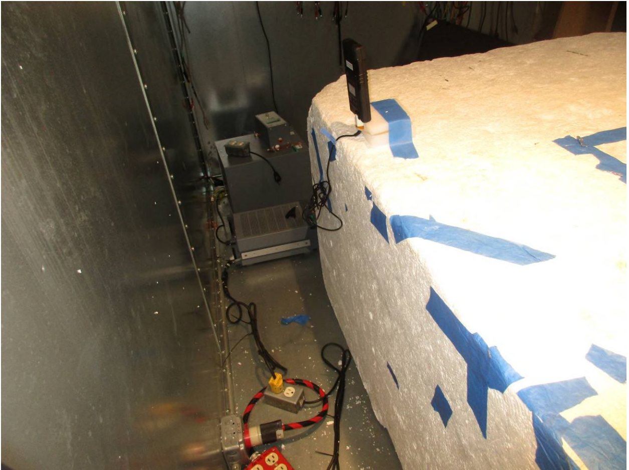
Figure 21: Power Line Conducted Emissions – Rear View
