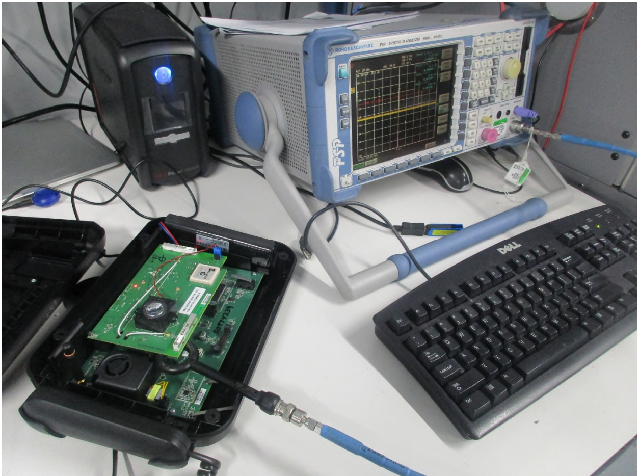
Figure 9: Near Field Measurements – 433.92 MHz
