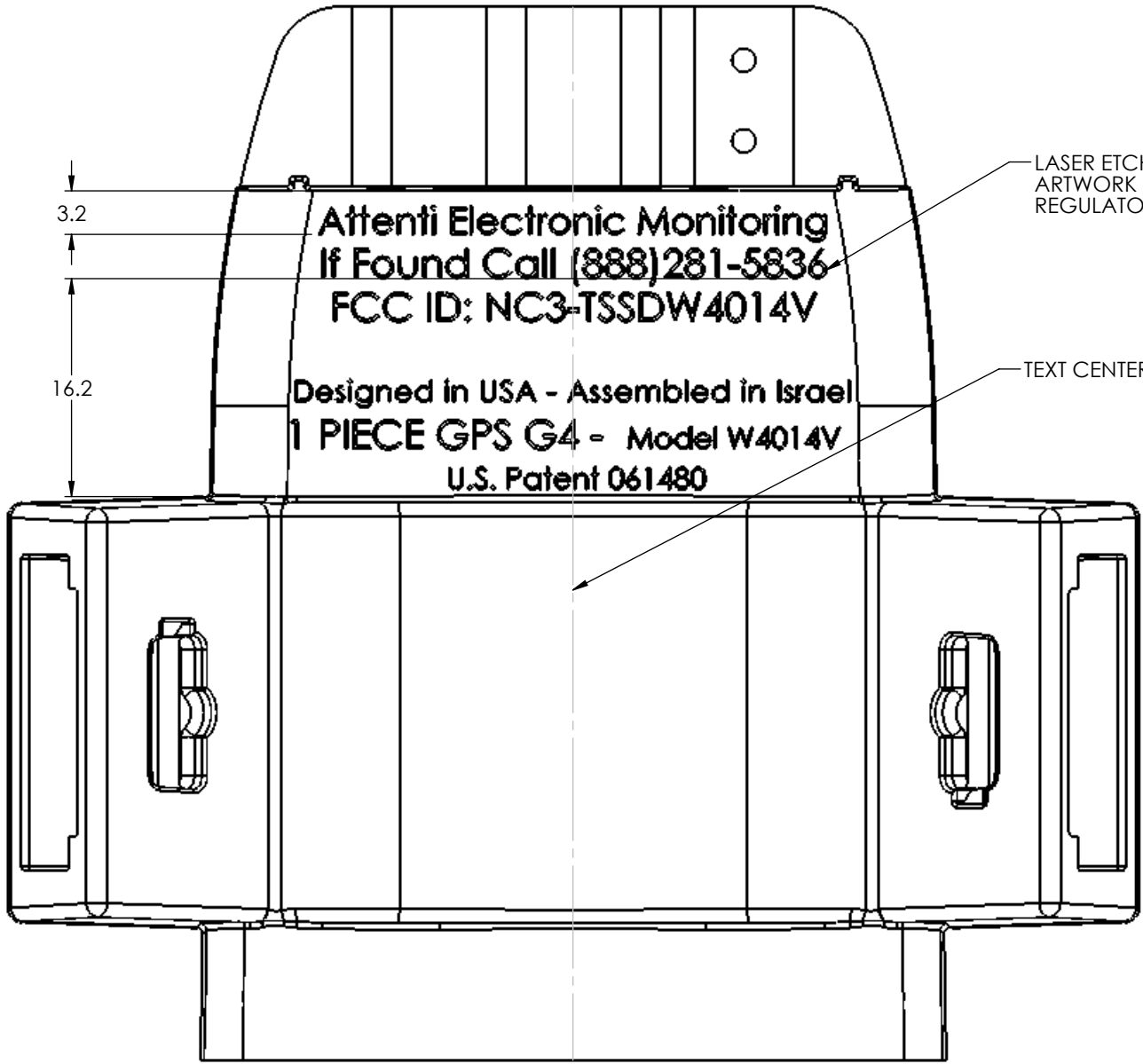
REAR/BACK VIEW
