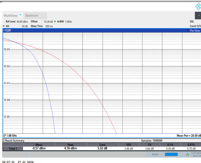
Band2-9400-2
