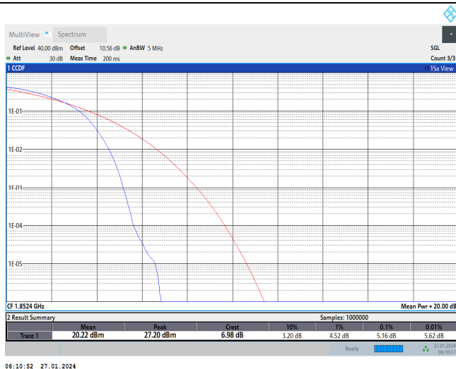
Band2-9262-5
