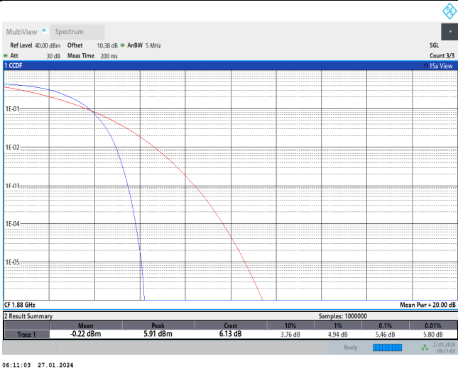
Band2-9400-5
