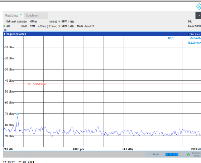
Band2-9538-1-0.009~0.15MHz
