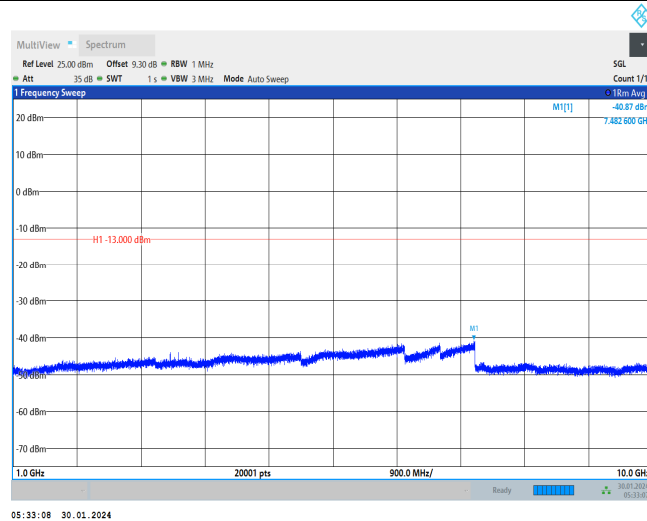
Band5-4233-4-1000~10000MHz
