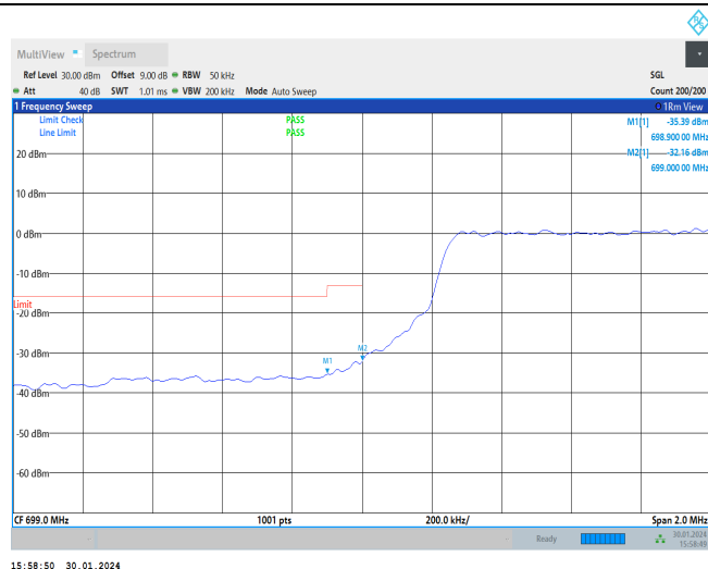
Band12-5MHz-QPSK-23155-1RB#24
