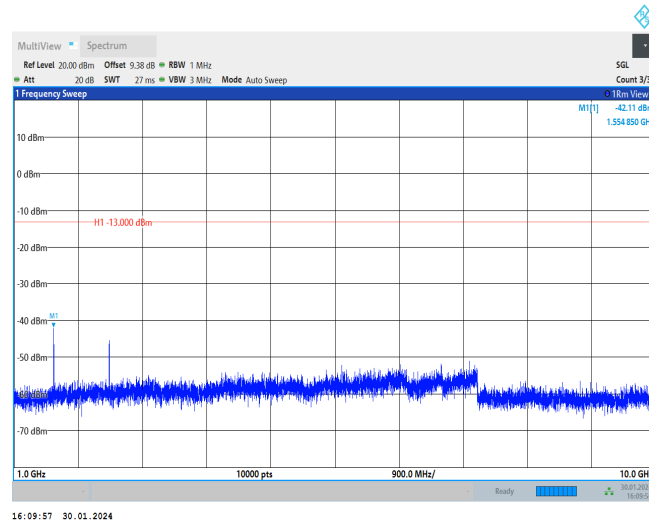
Band13-10MHz-QPSK-23230-1RB#0-Range2:1000~10000MHz
