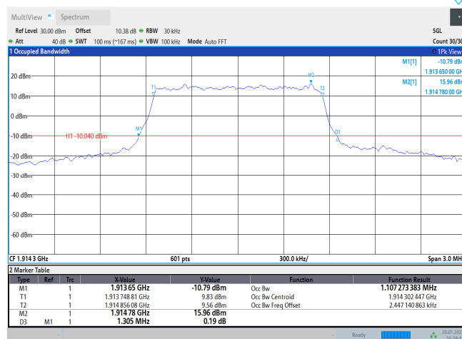
Band25-1.4MHz-QPSK-26683-6RB#0
