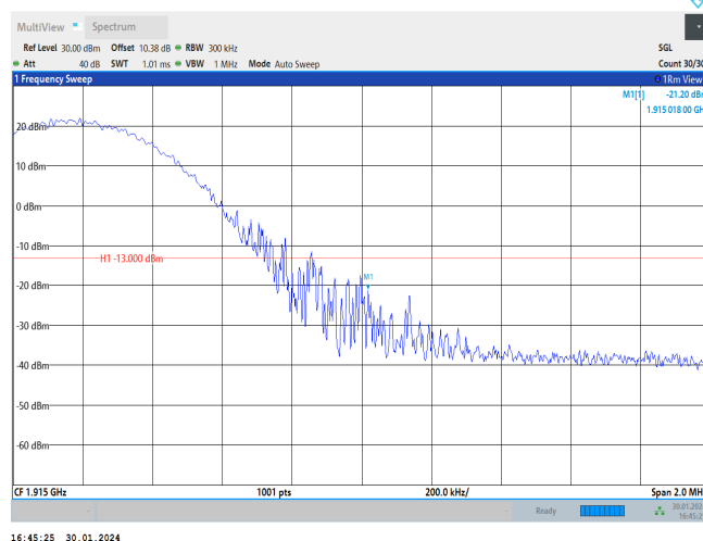
Band25-15MHz-QPSK-26615-75RB#0
