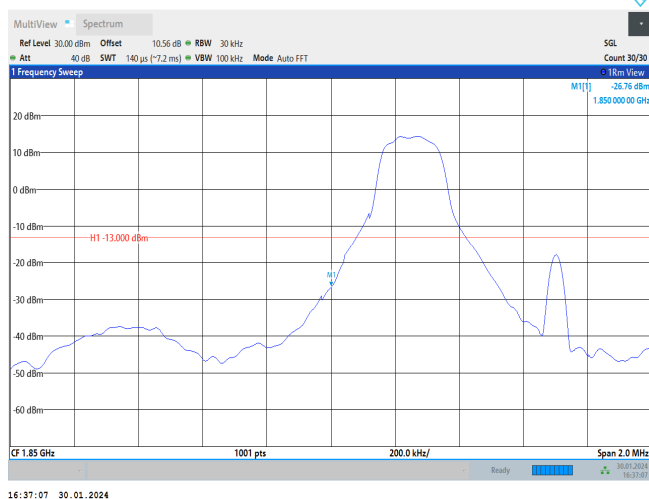
Band25-1.4MHz-QPSK-26047-6RB#0
