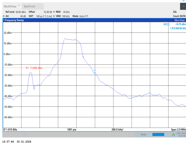
Band25-1.4MHz-QPSK-26683-1RB#5
