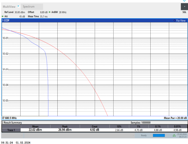
Band71-15MHz-QPSK-133297-75RB#0
