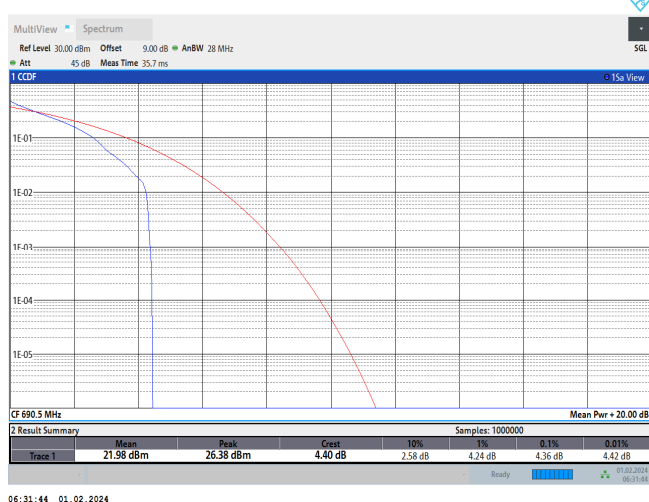
Band71-15MHz-QPSK-133397-75RB#0
