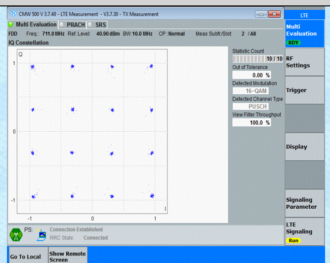
Band12-10MHz-16QAM-23130-27RB#0
