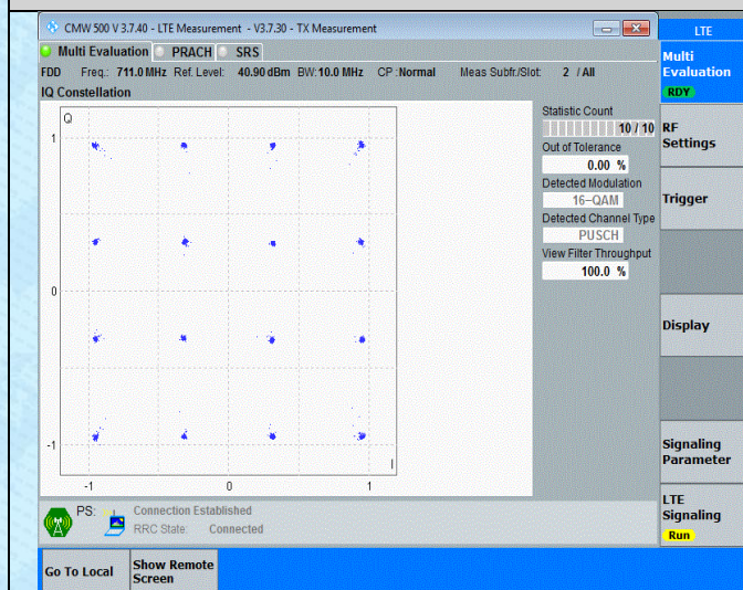
Band12-10MHz-16QAM-23130-27RB#23
