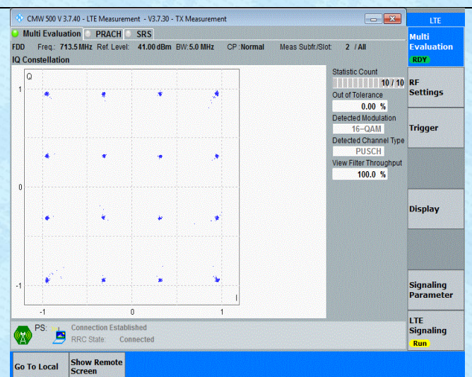
Band12-10MHz-QPSK-23095-50RB#0
