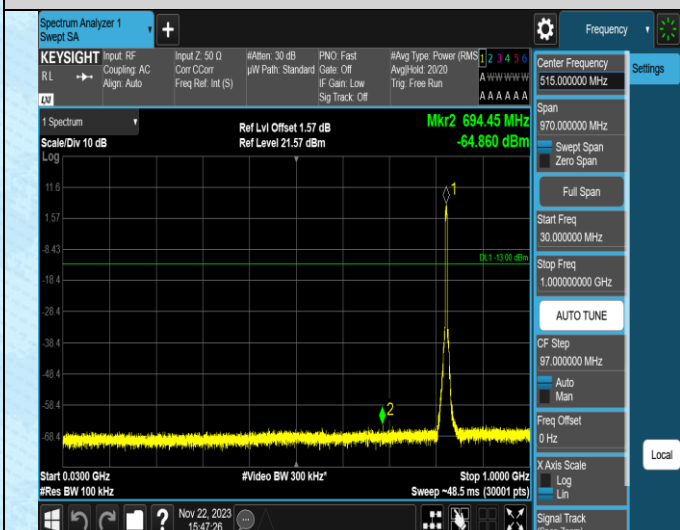
Band5-4182-1-30~1000MHz
