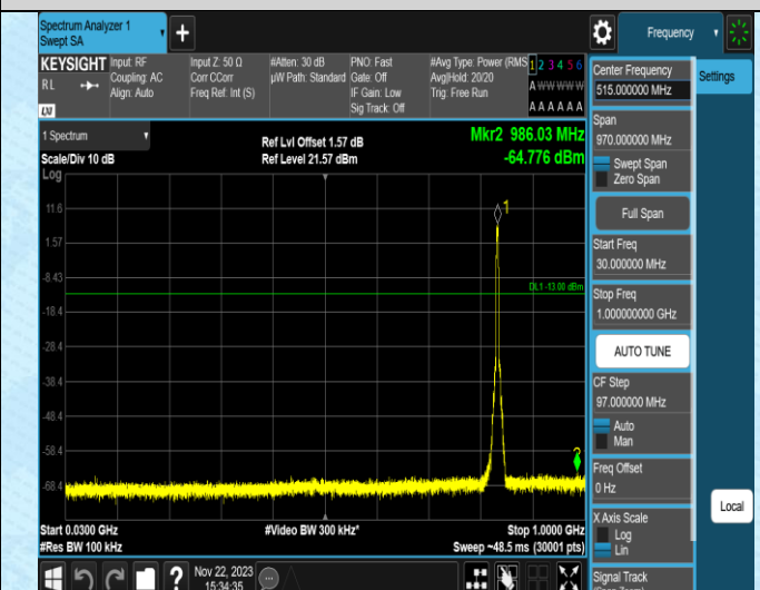
Band5-4233-30~1000MHz
