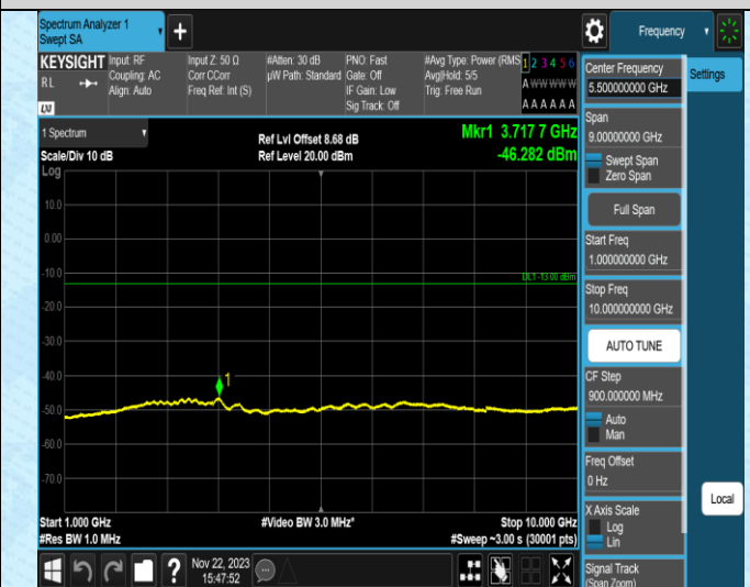
Band5-4182-1-1000~10000MHz
