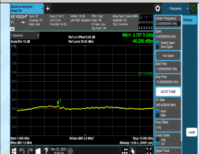
Band5-4233-1-1000~10000MHz
