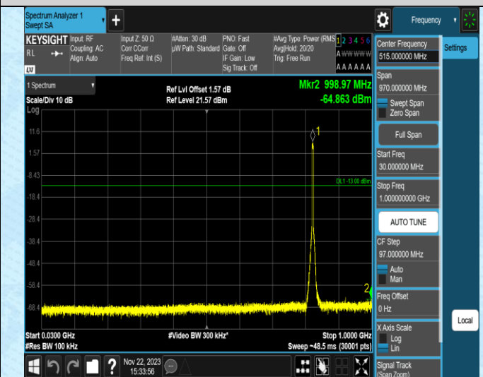
Band5-4182-30~1000MHz
