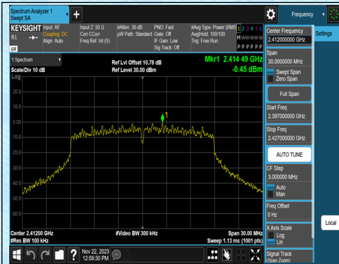
11N20SISO-Ant1-2412-0~Reference
