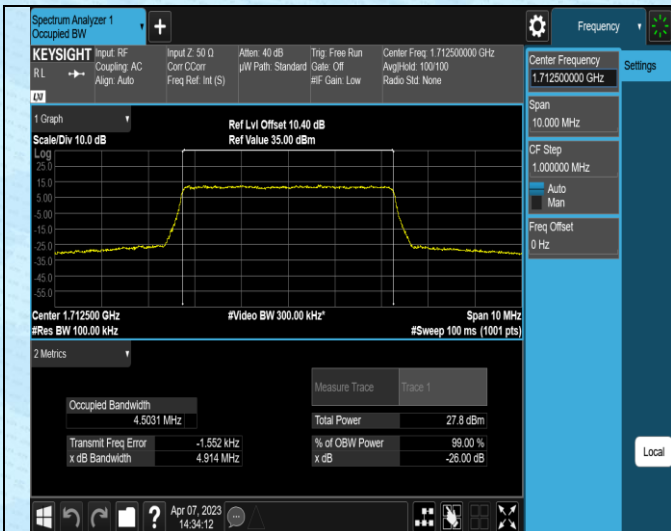
Band4-5MHz-QPSK-20375-25RB#0
