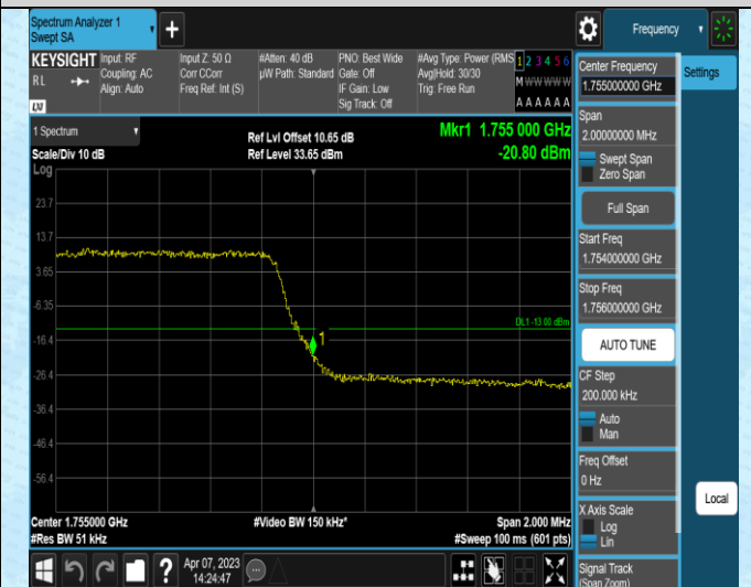
Band4-5MHz-QPSK-20375-25RB#0
