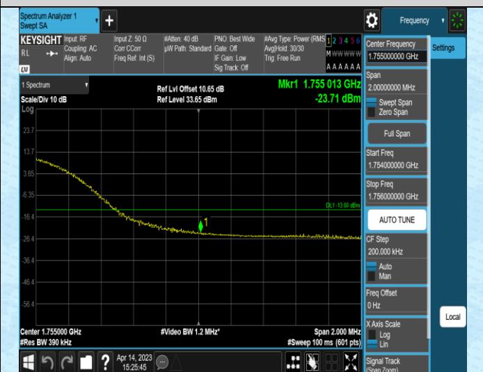
Band4-20MHz-16QAM-20300-27RB#73
