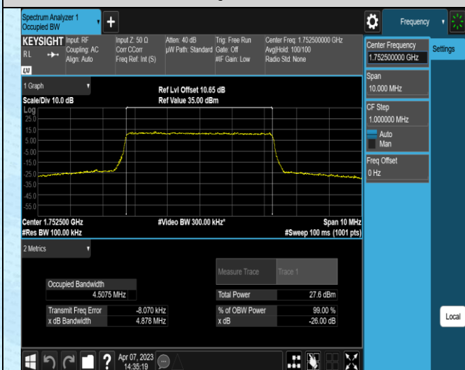
Band4-5MHz-16QAM-20175-25RB#0
