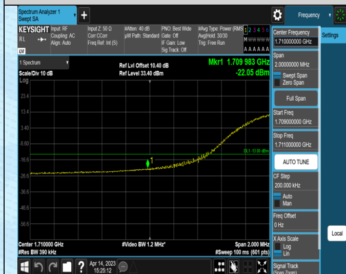
Band4-20MHz-16QAM-20050-27RB#0
