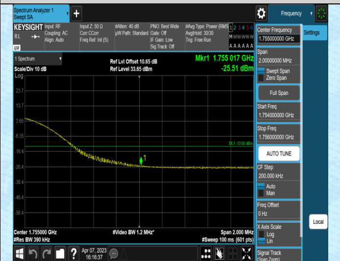
Band4-20MHz-16QAM-20300-27RB#73
