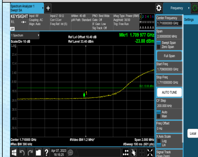
Band4-20MHz-16QAM-20050-27RB#0
