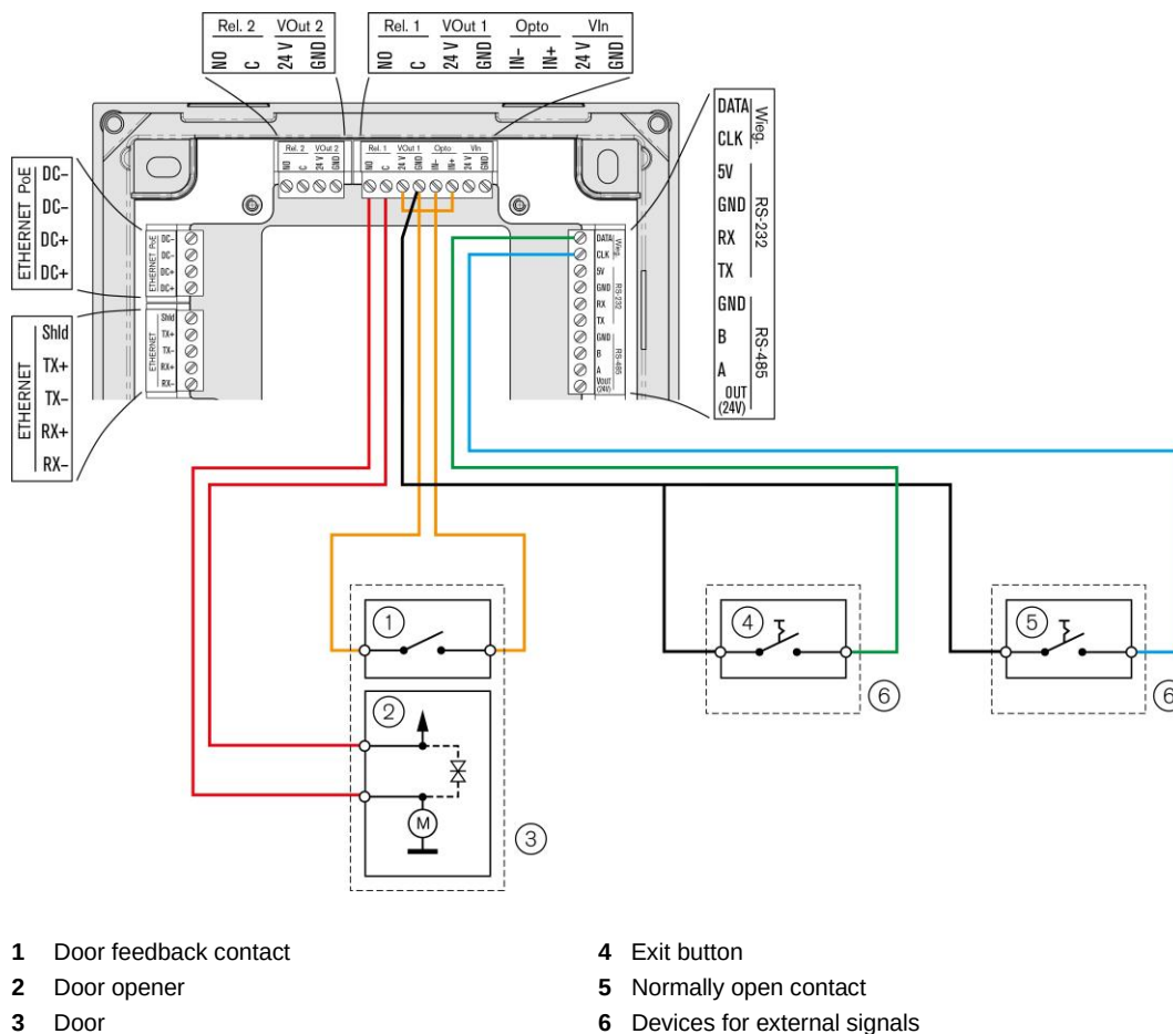
Figure 4.2 – Connection of the digital inputs and outputs (example)
