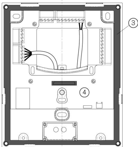
Figure 3.5 - Gasket and connector
