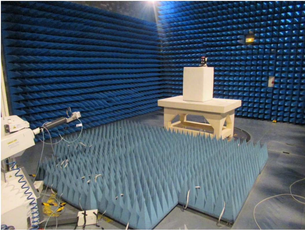
Test Setup Photo – Frequency stability , 20 dB Bandwidth and Occupied Bandwidth
