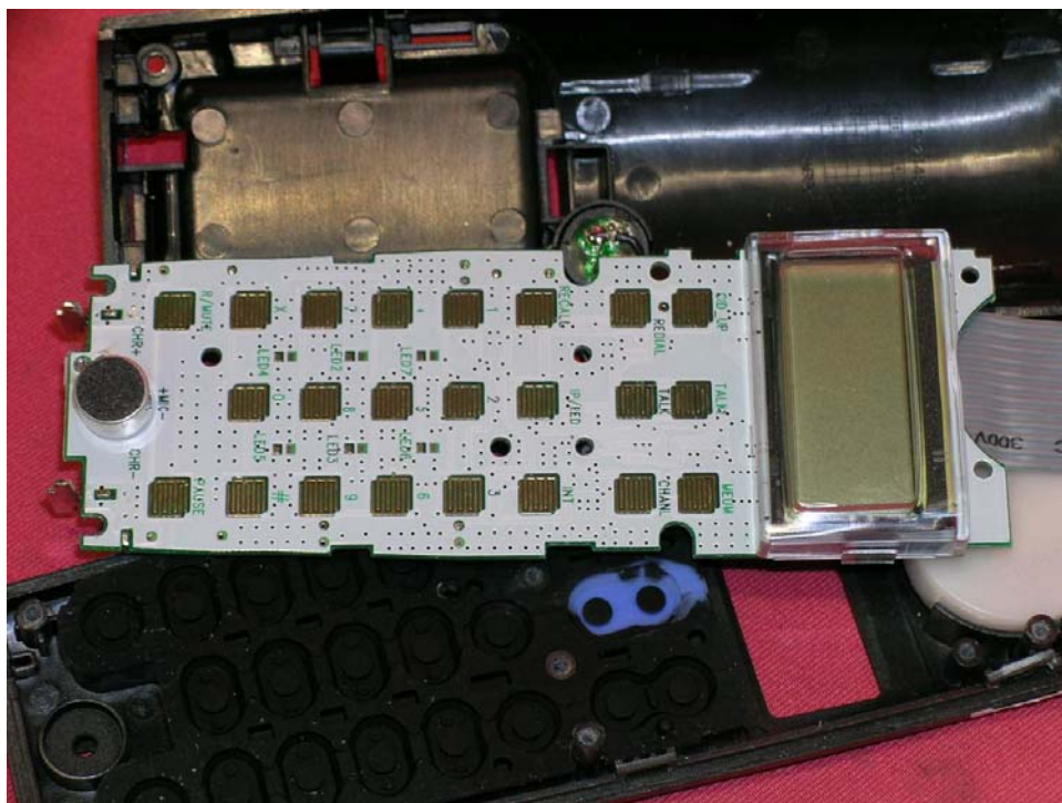
Handset display PCB front side
