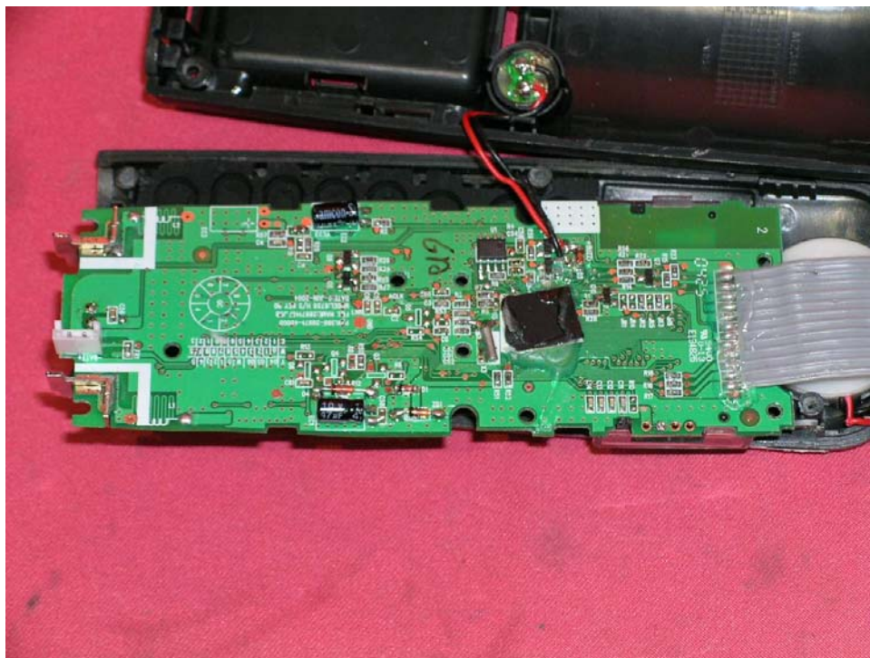
Handset display PCB rear side (View 1)
