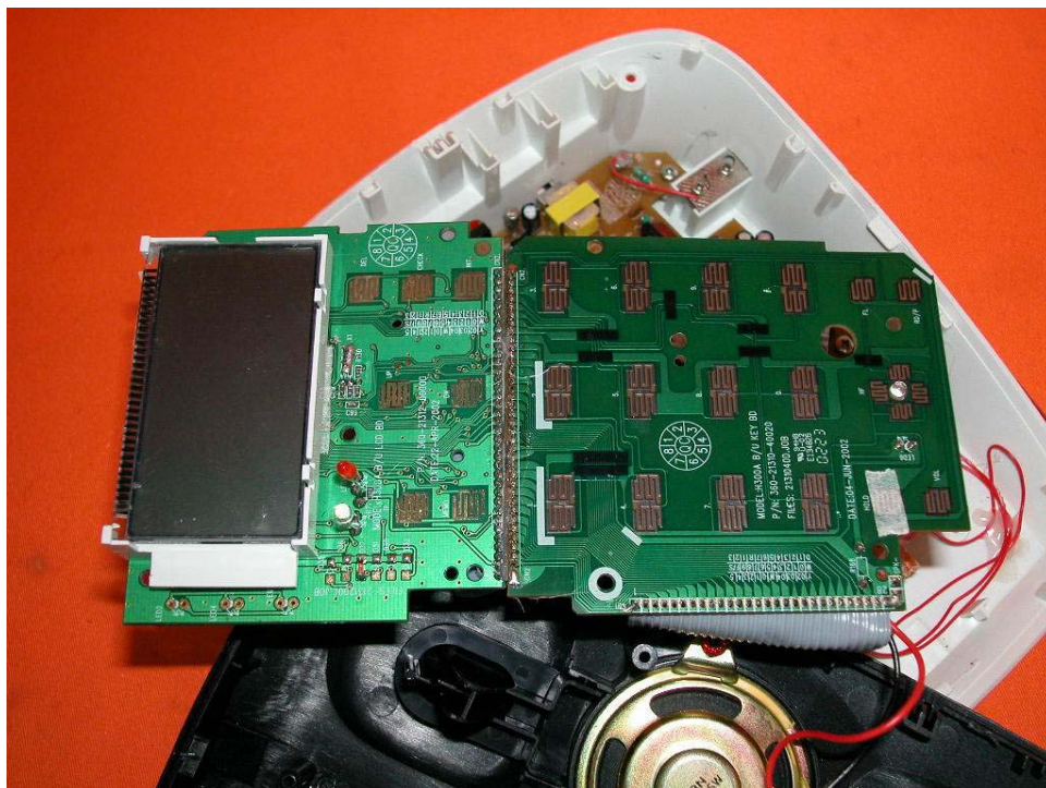
Base PCB display and keypad side
