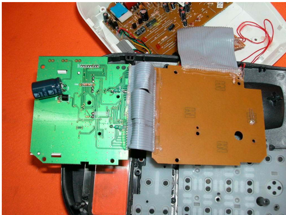
Base PCB display and keypad rear side
