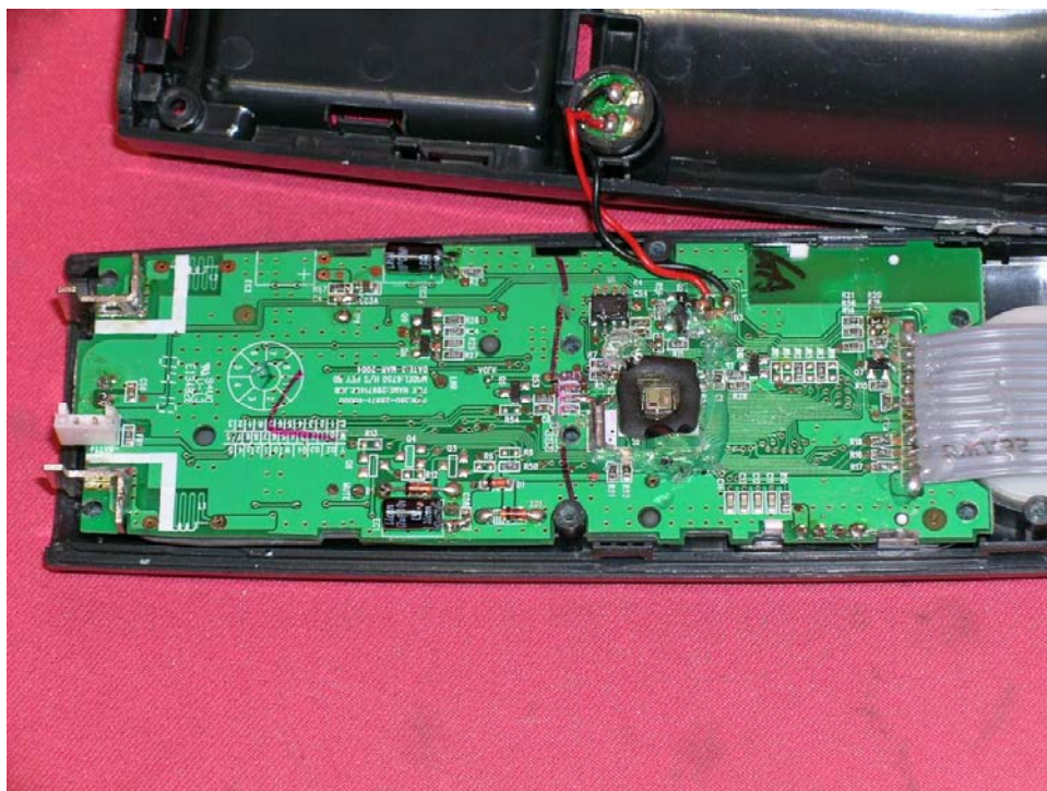
Handset Main PCB display rear side (View 2)
