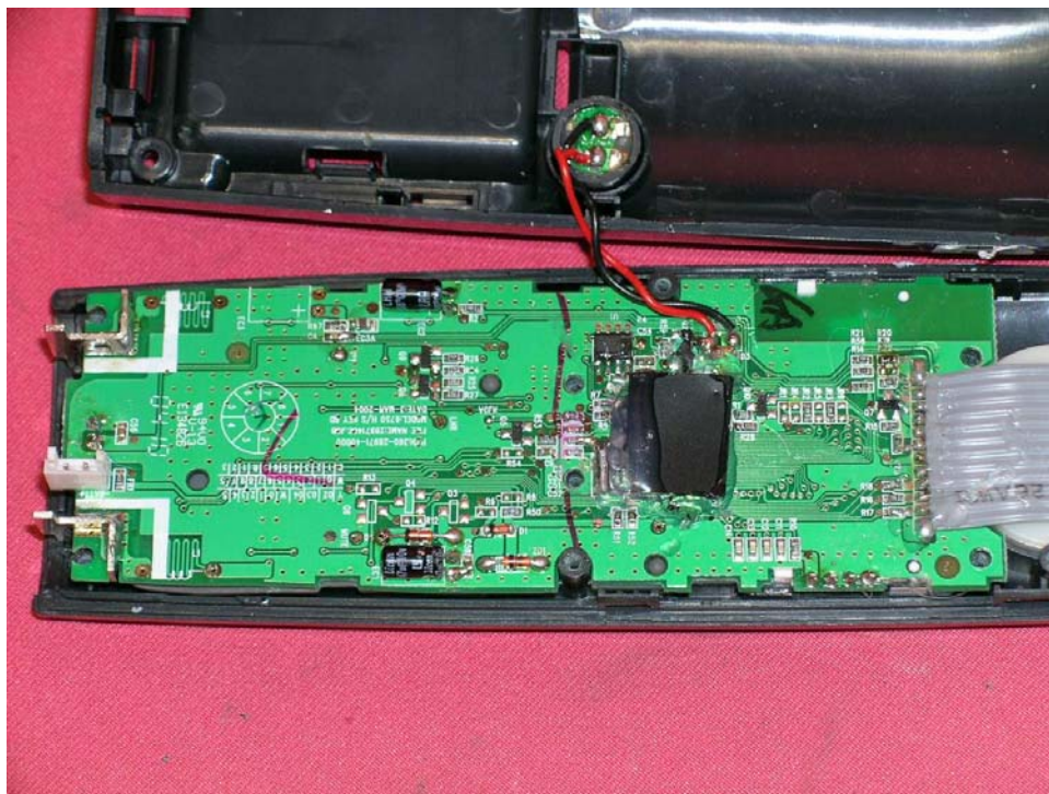
Handset Main PCB display rear side (View 1)
