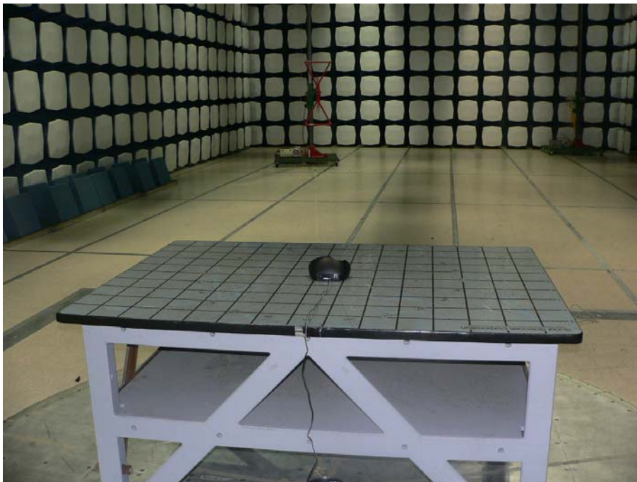
Radiated Emissions - TX Mode Spurious Emissions Rear View For Base Part of EUT
