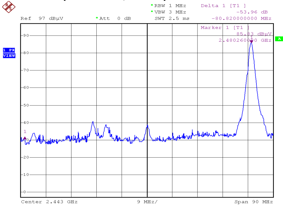
Plot B1A01 (KX-TG2130, 450mA)
