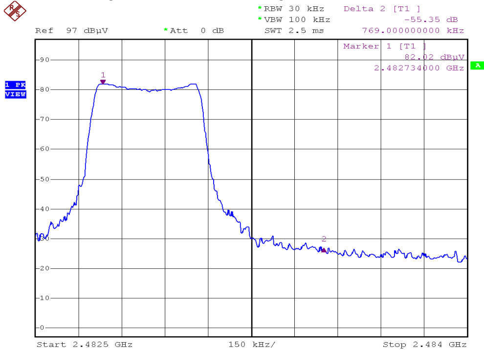
Plot B1B02 (KX-TG2130, 450mA)
