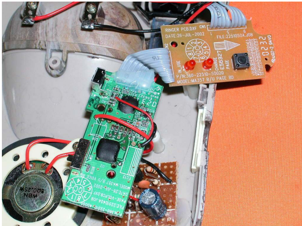
Base page key and melody key PCB comp side
