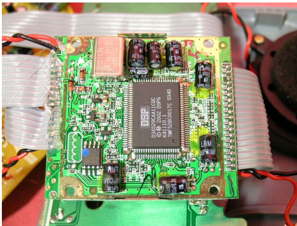
Base MCU PCB front side
