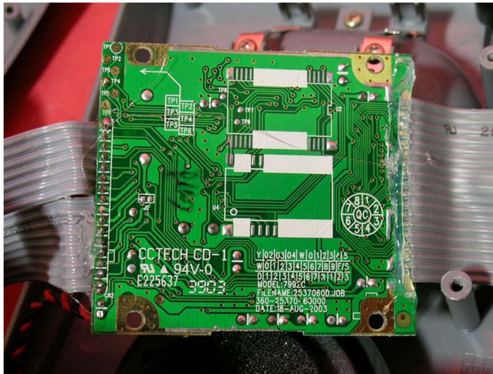
Base MCU PCB rear side
