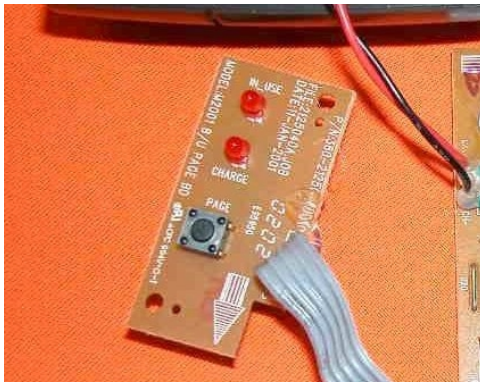
Base Page Key PCB comp side
