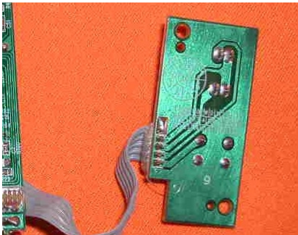
Base Page Key PCB solder side
