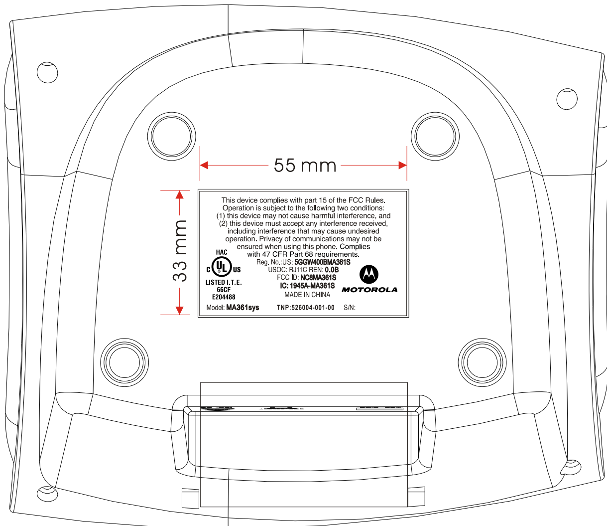
MA361sys BU LABEL DRAWING
