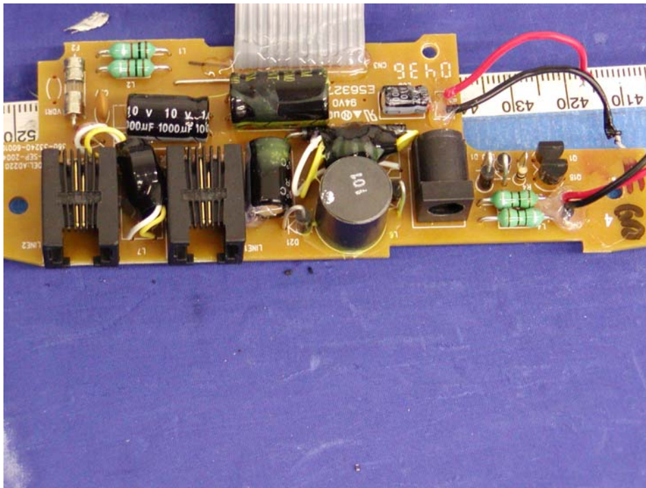
Base - Page Board Component View II
