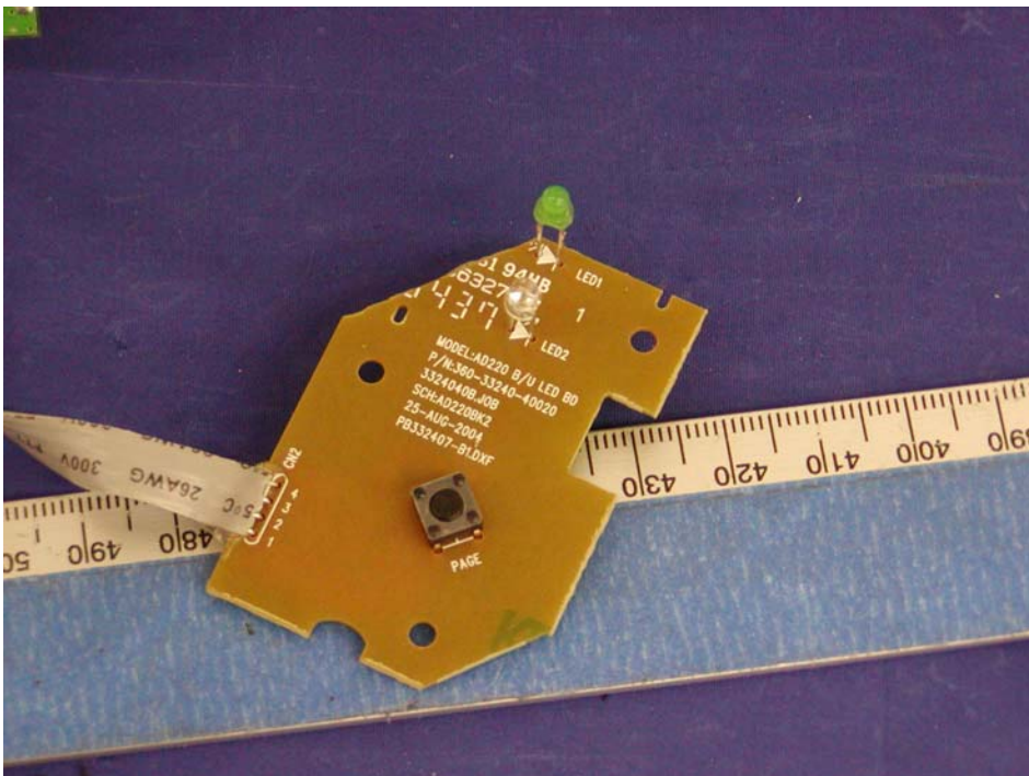
Base - Page Board Component View I
