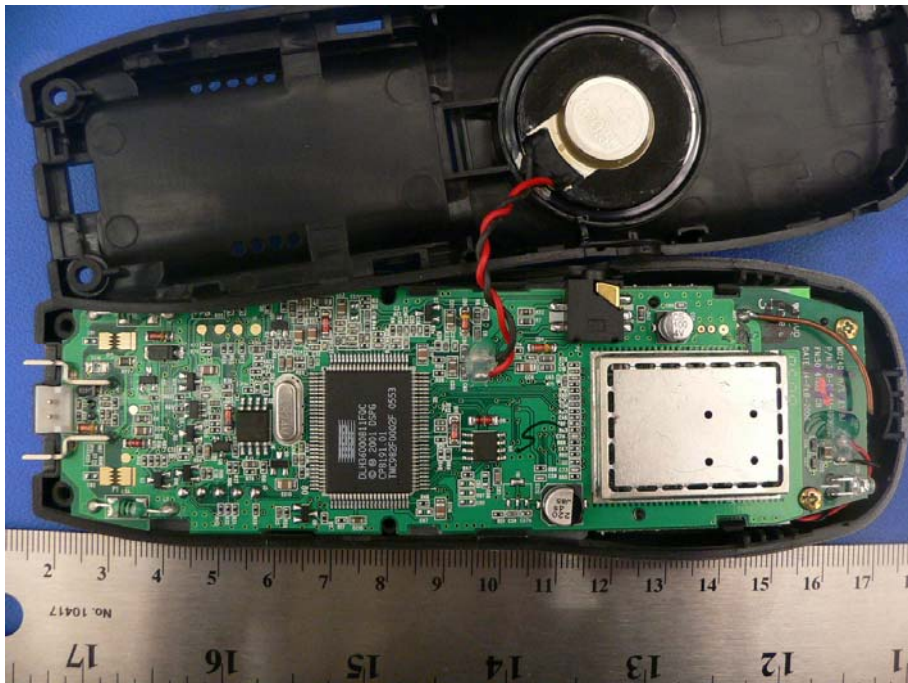
EUT –Chassis off View (Handset)
