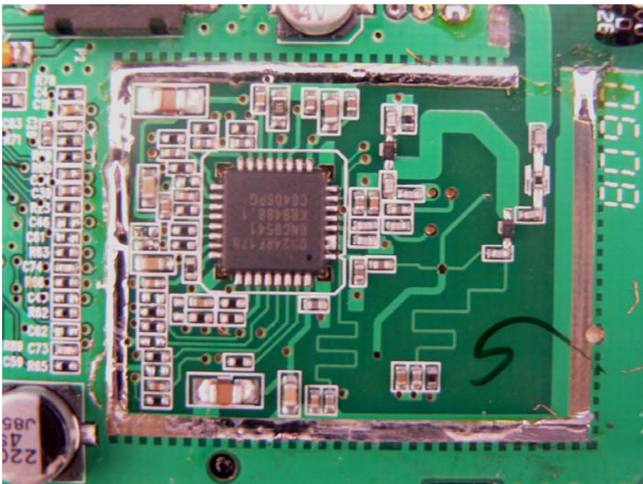
EUT –RF Shielding off View (Handset)
