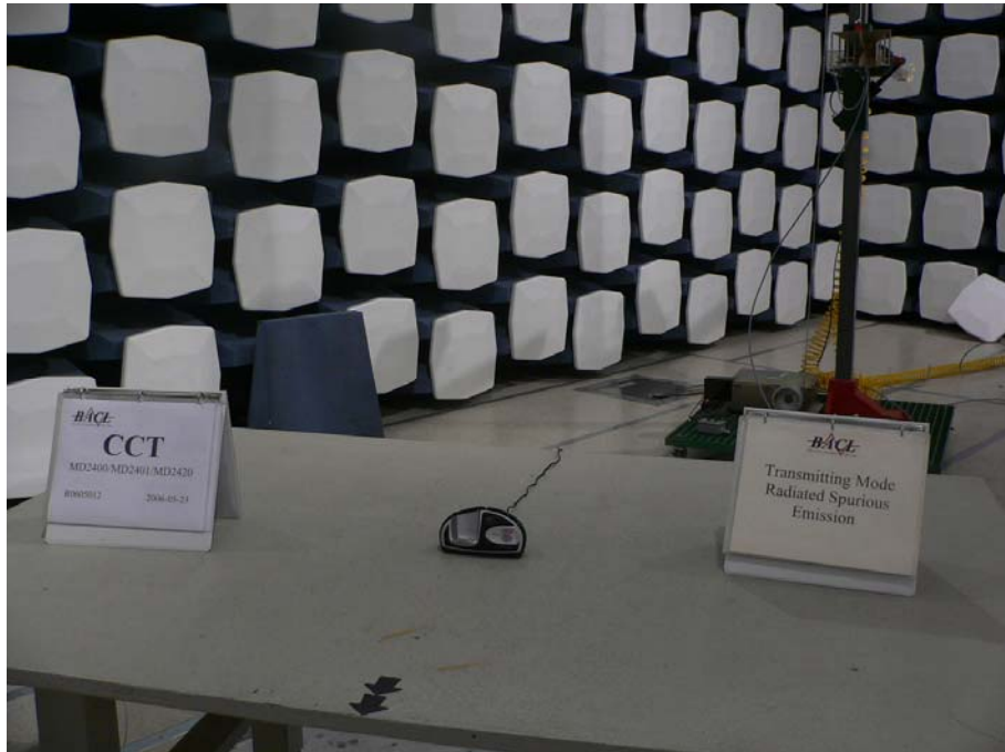
TX Mode Spurious Emissions Front View For Base Part of EUT
