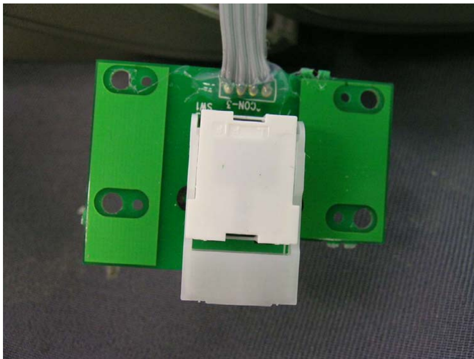
Base hook switch front side
