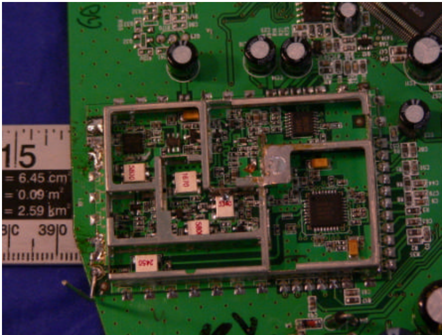
Base – TX View
