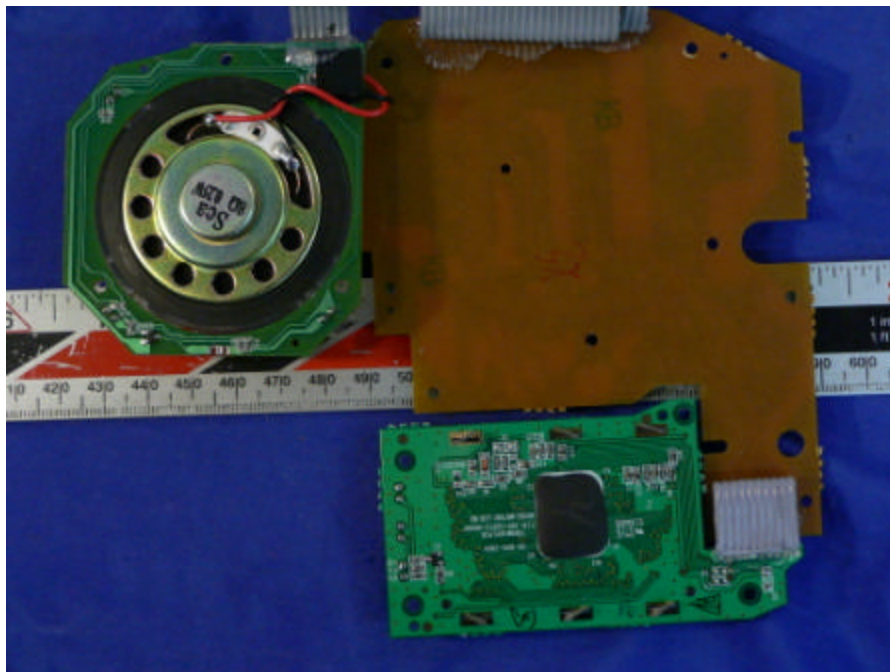
Base– LCD Keypad Board Component View
