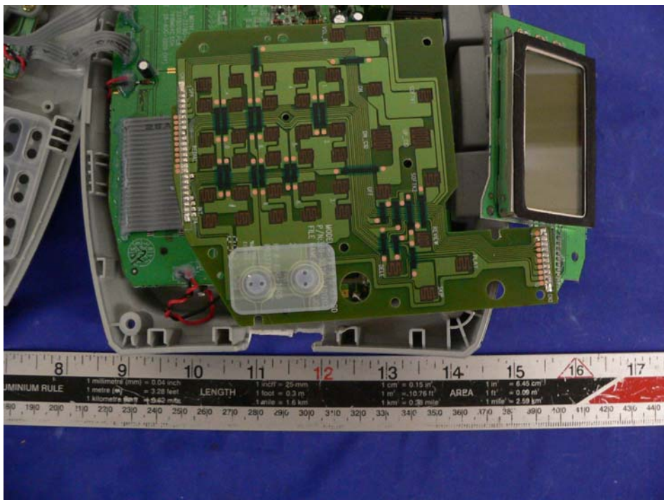
EUT – Keypad with LCD View
