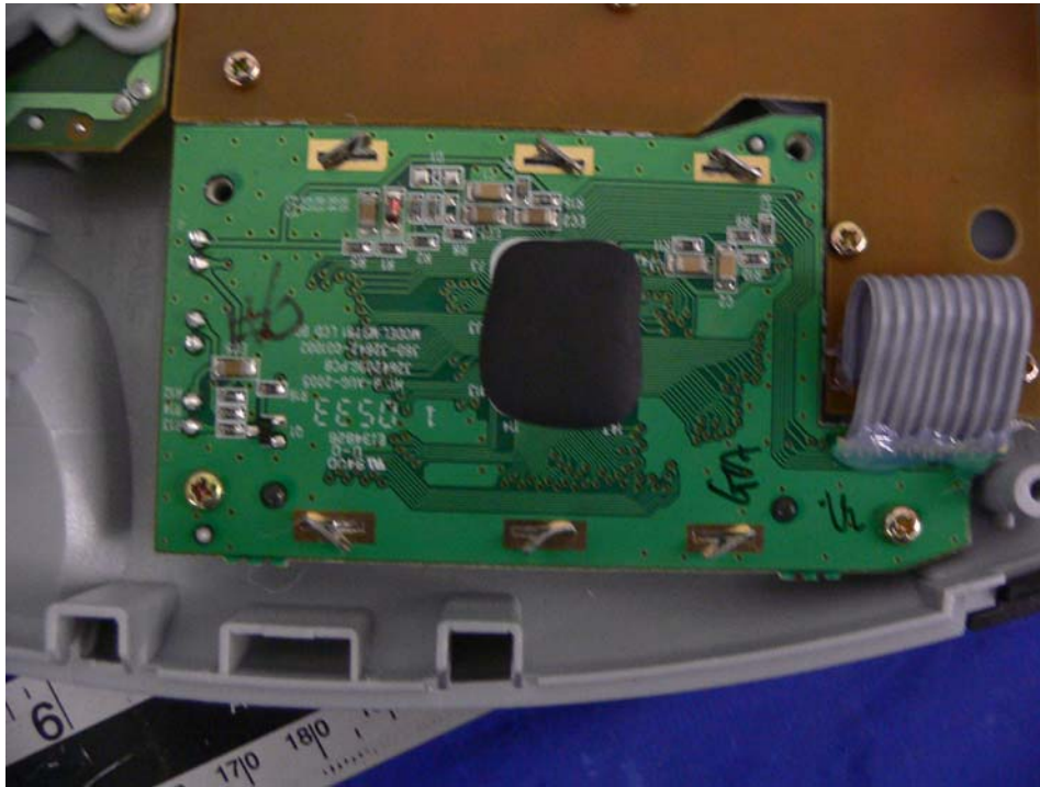
EUT – Caller ID Board View
