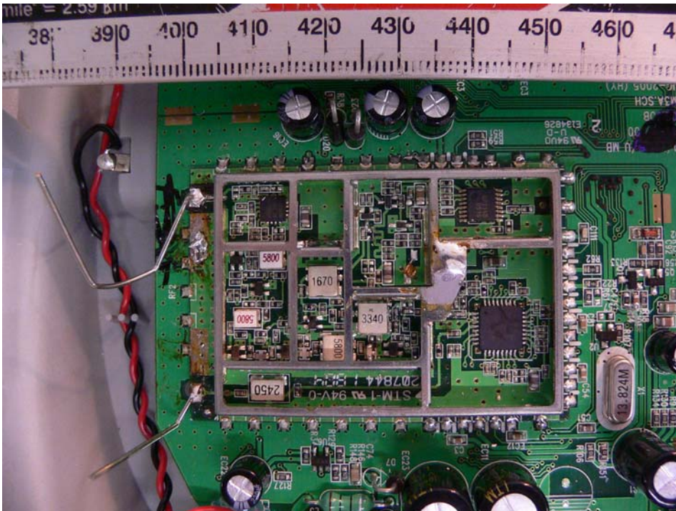
EUT – RF Antenna View
