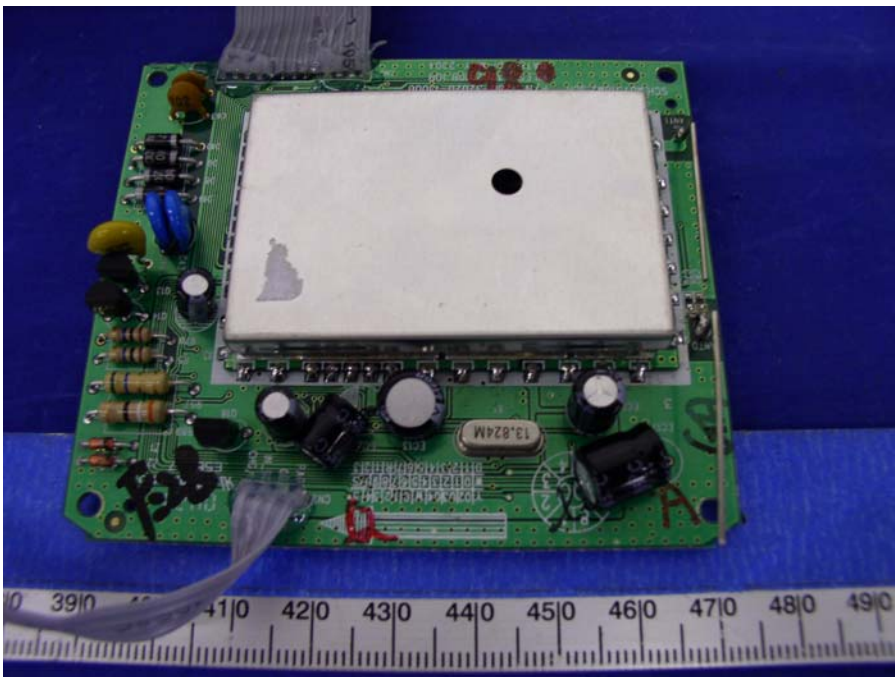
Base MD751 - Main Board Component View with Shielding
