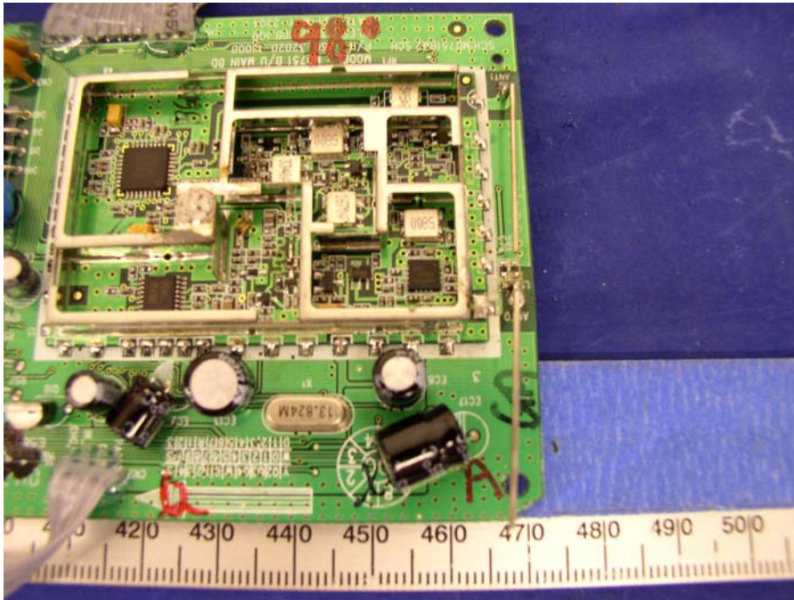
Base MD751 - Transceiver Component View
