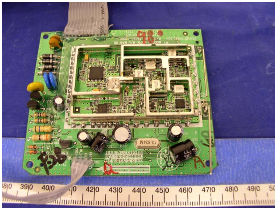
Base MD751 - Main Board Component View without Shielding
