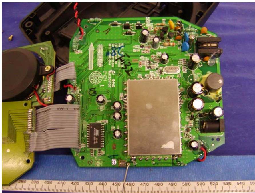
Base MD761 - Main Board Component View with Shielding
