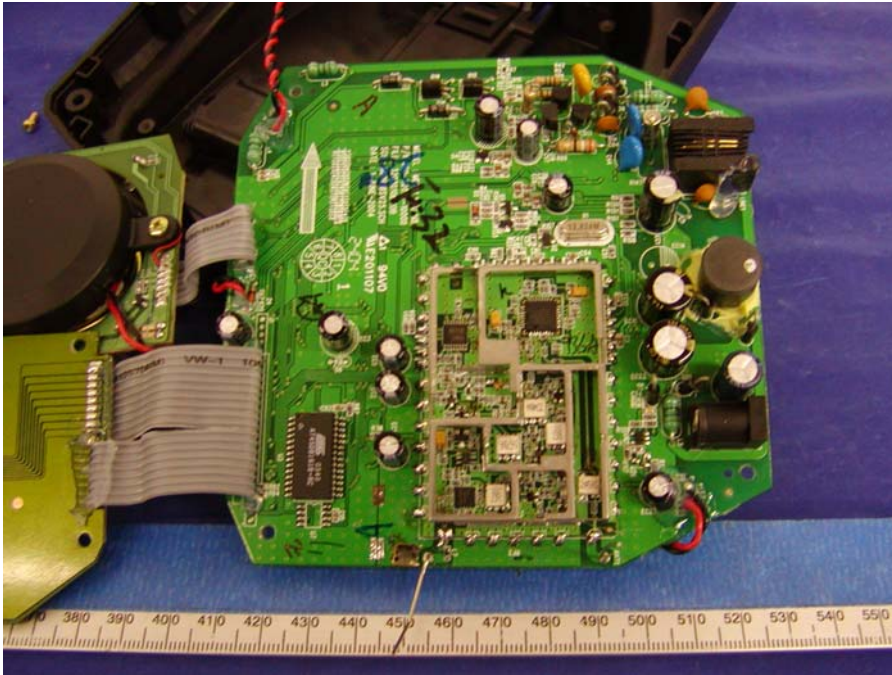
Base MD761 - Main Board Component View without Shielding
