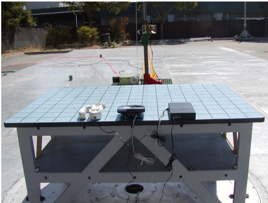
MD761 Base Radiated Emission - Rear View
