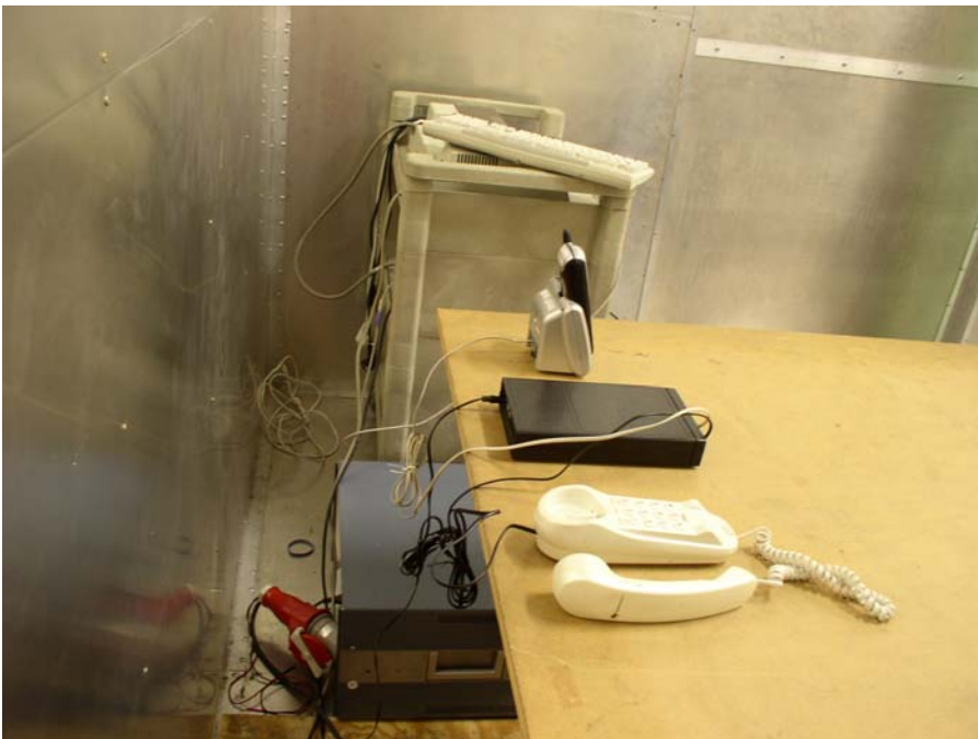
MD751 Conducted Emission - Side View
