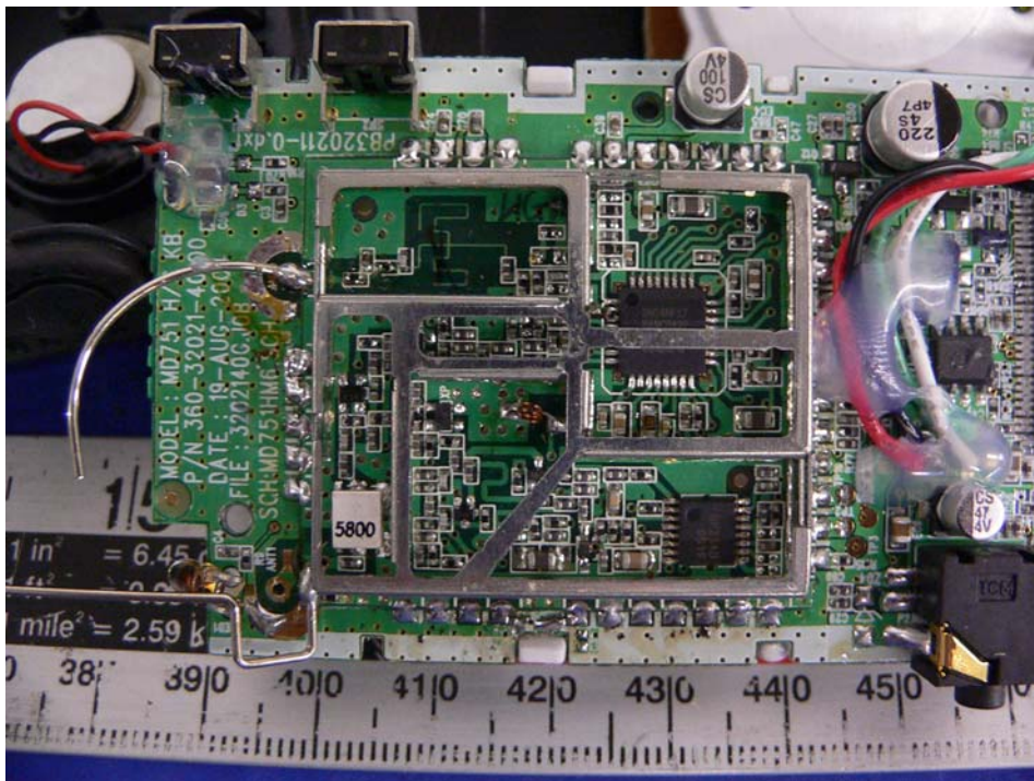
EUT - Transceiver Component View
