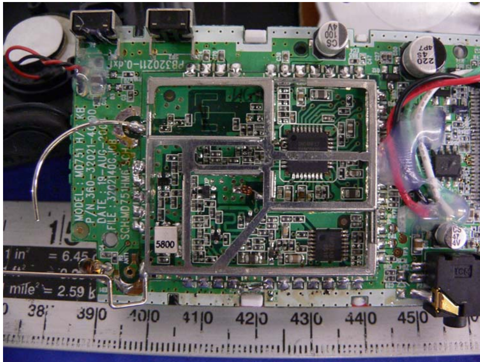
EUT – RF Closed Cover Off Antenna View
