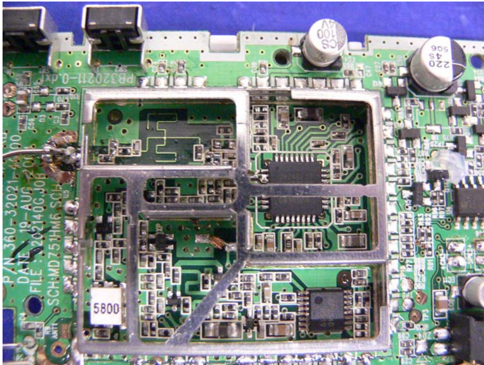
EUT - TX View
