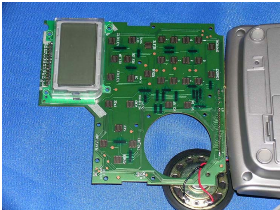
Base TAD and keypad PCB front side
