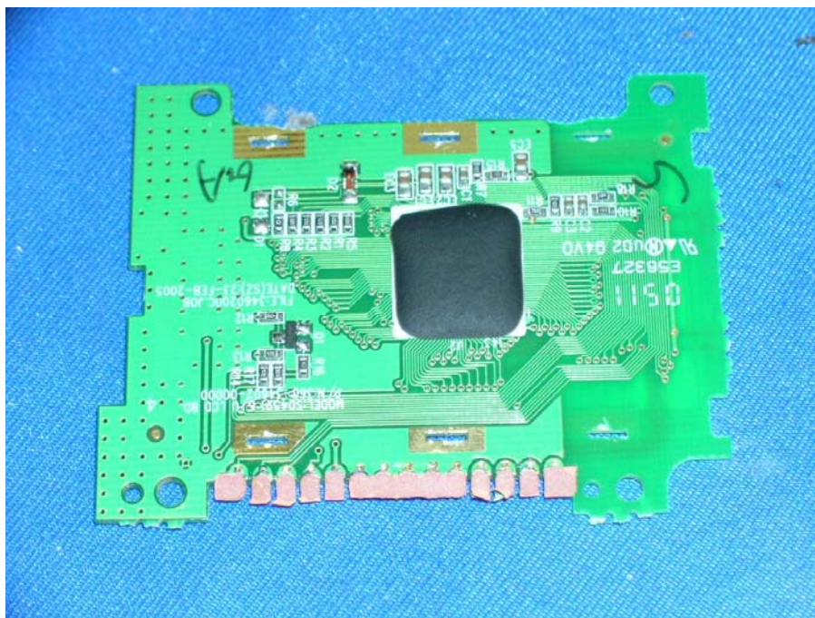
Base LCD Display and Keypad rear side (View 2)
