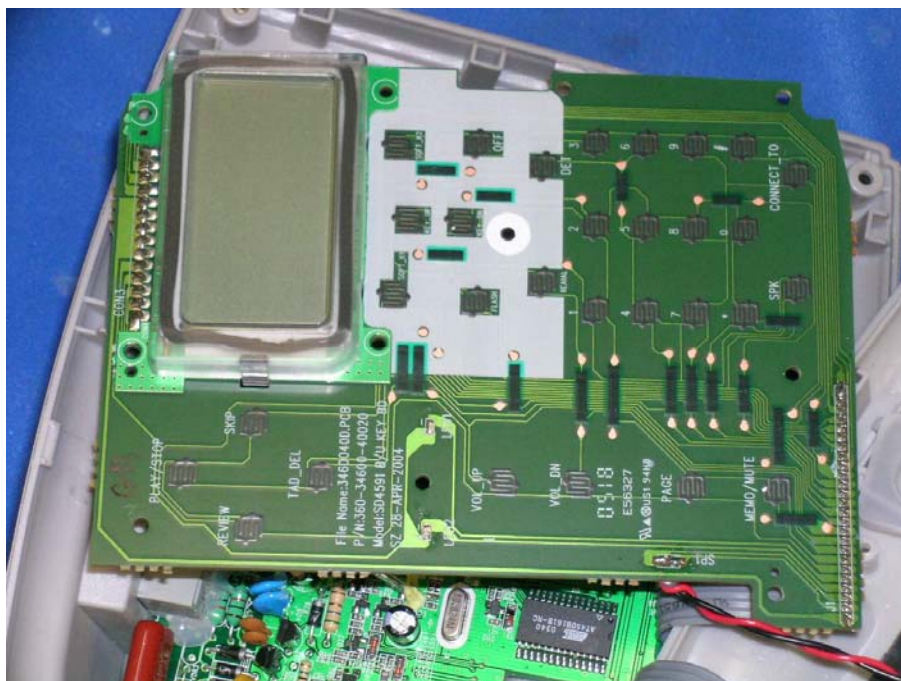
Base LCD Display and Keypad front side
