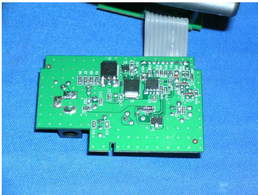
Cell Dock AC Jack solder side
