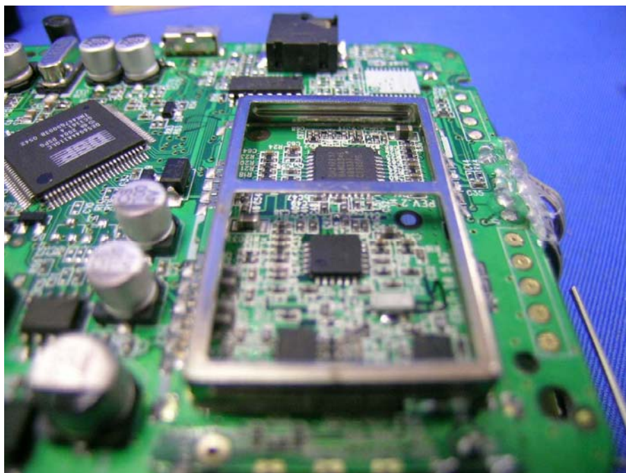
Cell Dock 5.8GHz RF module comp side (View 2)
