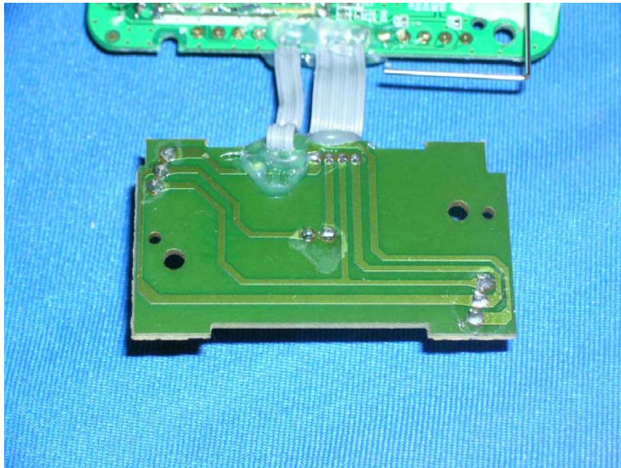
Cell Dock Bluetooth button & LEDs rear side
