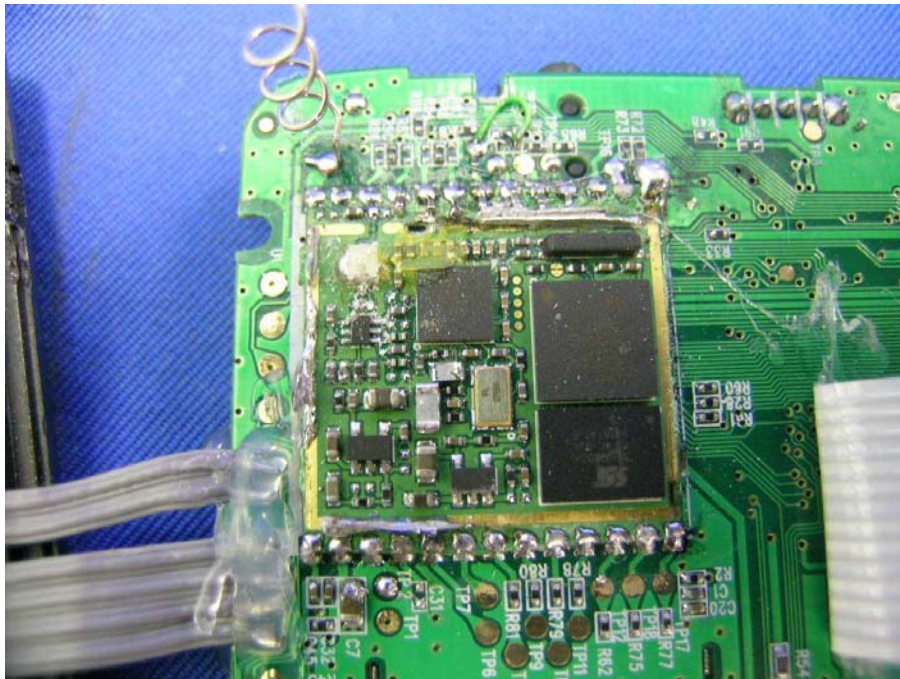
Cell Dock 2.4GHz RF module comp side
