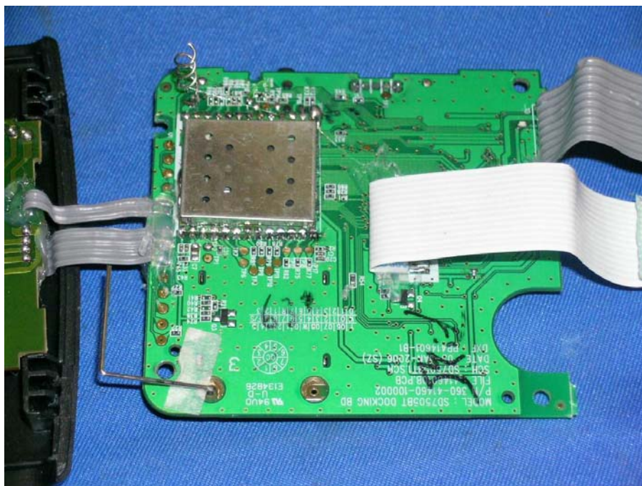
Cell Dock Main PCB solder side (View 2)
