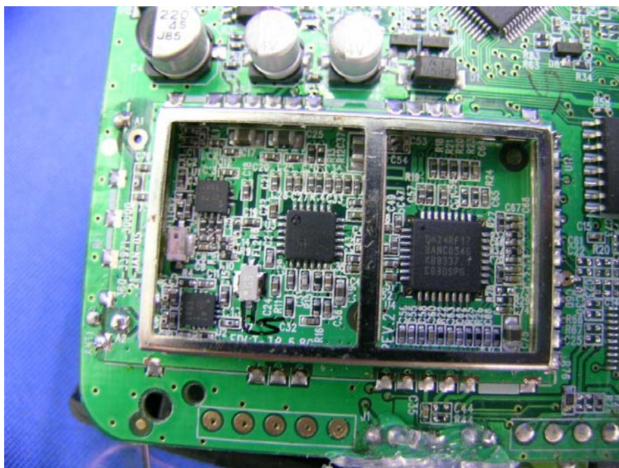
Cell Dock 5.8GHz RF module comp side (View 1)
