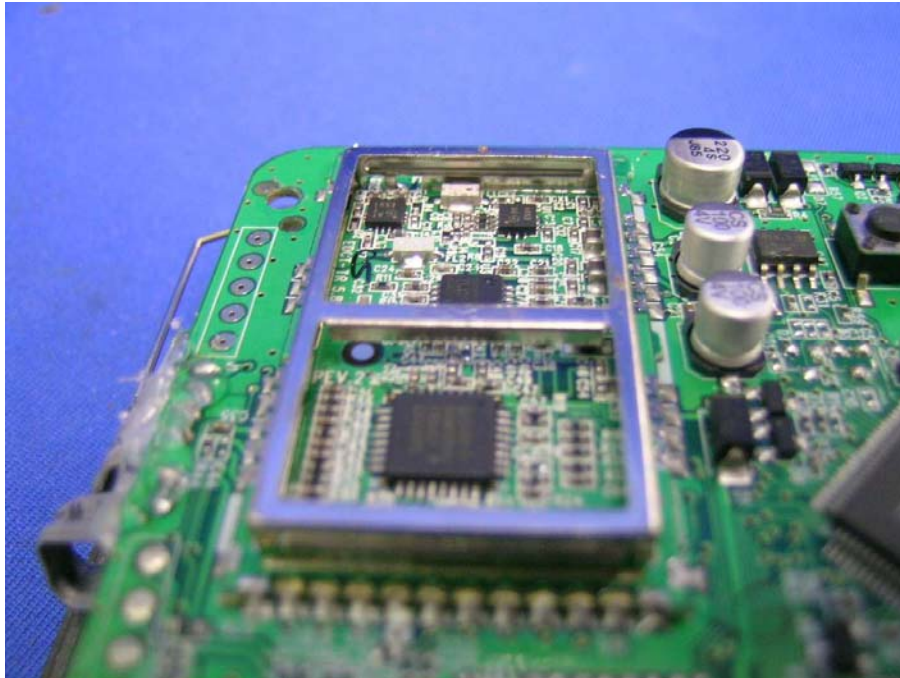
Cell Dock 5.8GHz RF module comp side (View 3)
