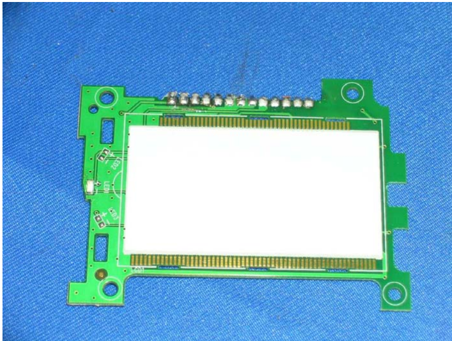
Base LCD display front side (View 2)
