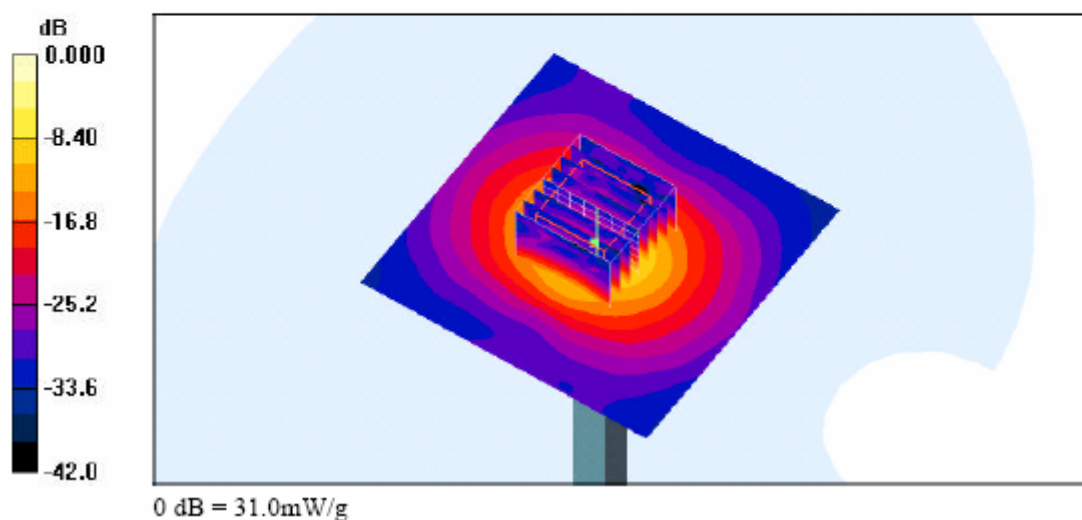
Body-Tissue-Simulating-Liquid 5.8GHz
