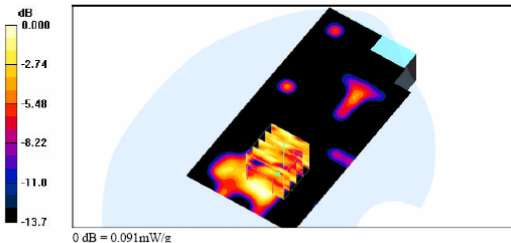
Body-SAR Test Result for Flat Position – Channel 1
