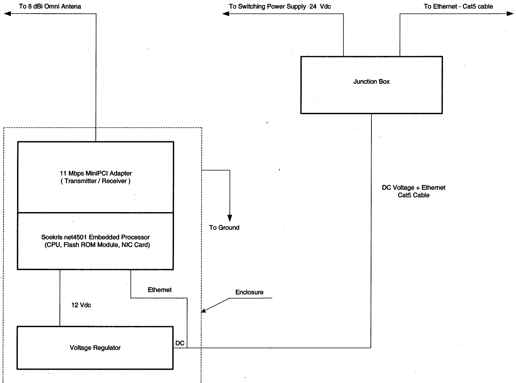
Figure 1. Block Diagram of Wireless Outdoor Mount Ethernet NCBSL9101 Bridge
