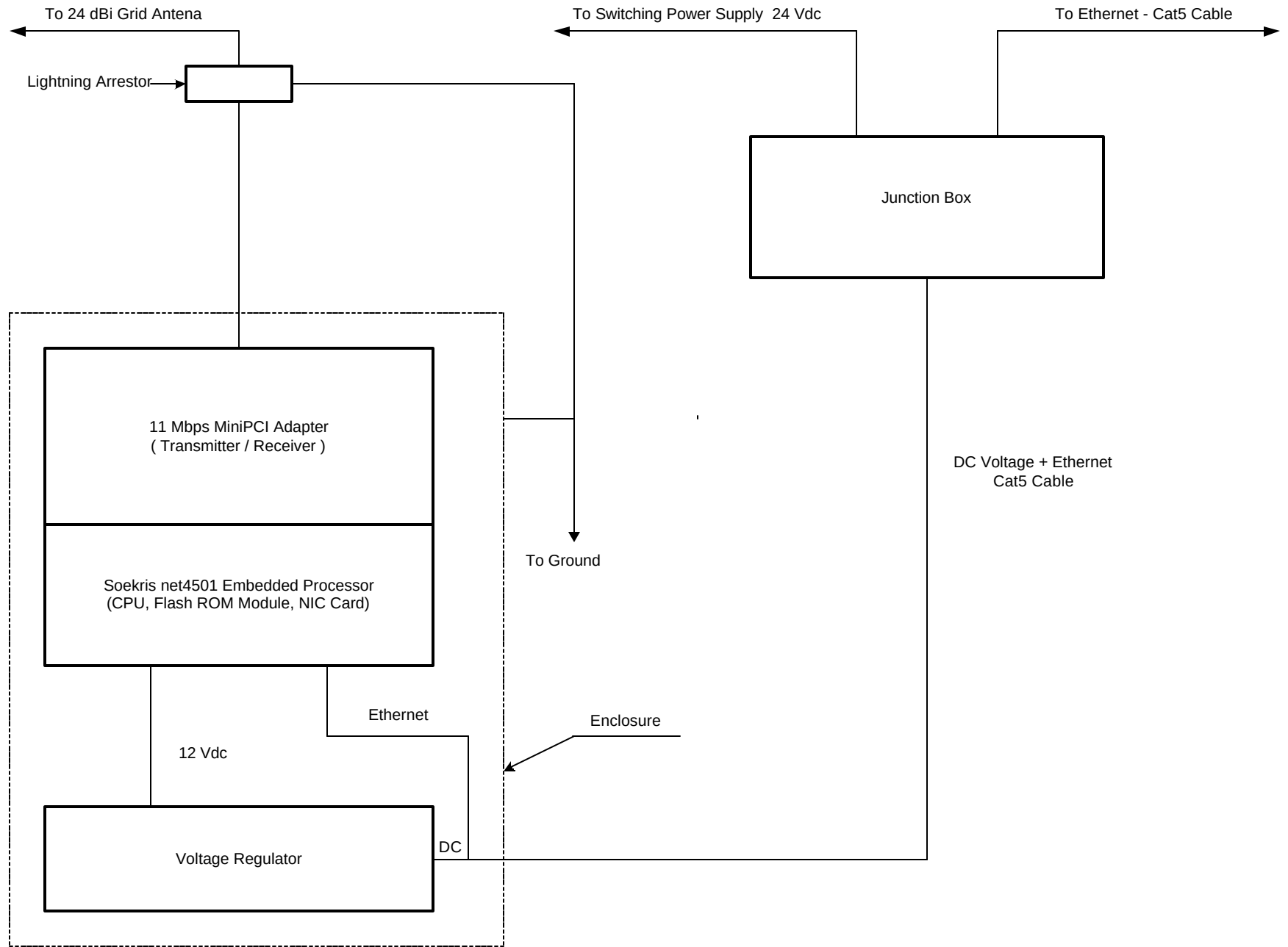
Figure 1. Block Diagram of Wireless Outdoor Mount Ethernet NCBSL9102A Bridge
